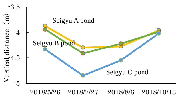
Fig. 47 Elevation of bed in Seigyu ponds
