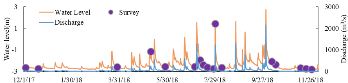
Fig. 5 Hydrograph of 2018
