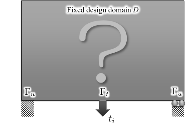
Fig. 8 Fixed design domain and boundary conditions of design model 2
