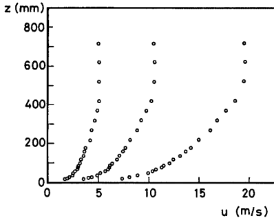
Fig. 4 Mean wind speed profiles.
