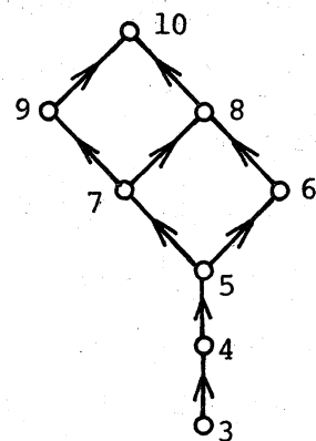
Fig.2. Example 2. (a) G_i and G_v . E_j = \{j\} , E_e = \{e\} .
