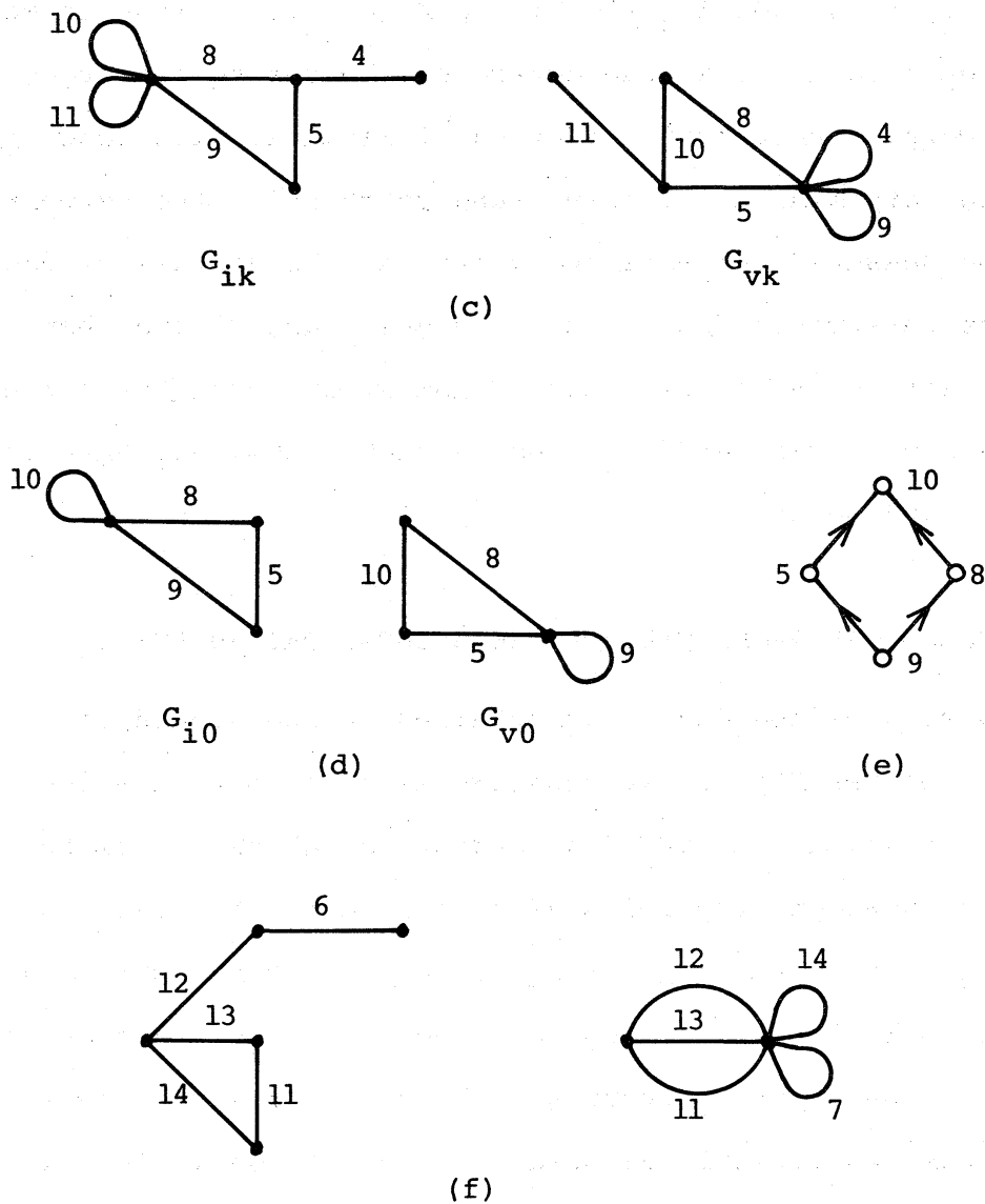
Fig.1. Example 1(continued) (c) G_{ik} and G_{vk} . (d) G_{i0} and G_{v0} . (e) partial ordering of the edges in E_0 . (f) G_i \cdot (E_u \oplus E_e \oplus E_2) and G_v \cdot (E_u \oplus E_j \oplus E_2)
