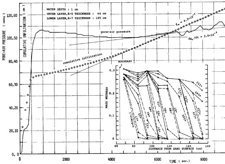
Fig. 25. Cumulative infiltration amount, pore-air pressure and distribution of moisture in two layered sand system (upper layer: sand K-5, lower layer: sand K-7).
