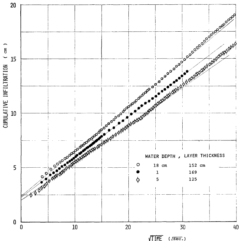
Fig. 5. Cumulative infiltration amount as a function of (time) ^{1/2} in column of sand K-7.
