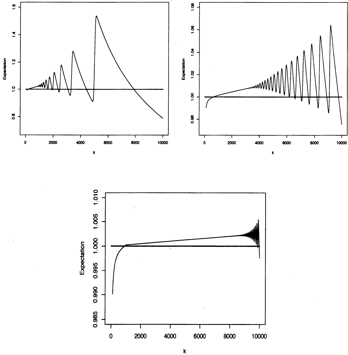
Figure 3: The mean value function of the Hill estimator \hat{\alpha}_{k,l}^{-1} for a sample of size n = 10\,000 of discretized Pareto distributed random variables X_1^{(l)}, \dots, X_n^{(l)} with parameter \alpha = 1 . Top left: l = 0 . Top right: l = 1 . Bottom: l = 2 .
