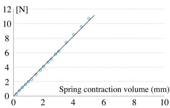
Fig. 8b Validation experiment 2-2. compression coil spring (1.2-10-41)
