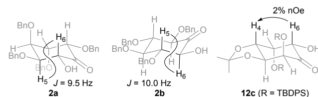
Figure 2. Determination of the stereochemistry of inososes.
