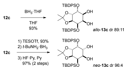
Scheme 6. Stereoselective reduction of 12c .
