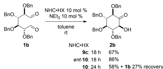
Scheme 2. Reaction with 1b .
