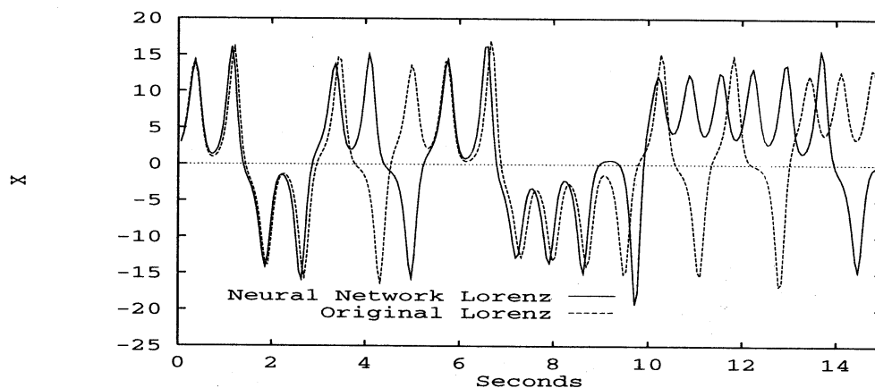
(a) 250 step 予測 (Hidden 4, Evidence = 4585)
