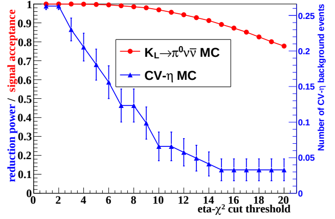
Figure 6.57: Signal acceptance (red) and CV- \eta background reduction power (blue) as a function of eta- \chi^2 cut threshold. The right blue axis represents the corresponding number of CV- \eta background events for the blue graph.
