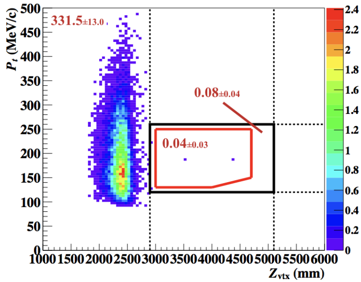
Figure 6.51: P_t - Z_{\text{vtx}} distributions of the upstream- \pi^0 background events after all the cuts imposed. The numbers in red indicate the number of events in each region bounded by lines.
