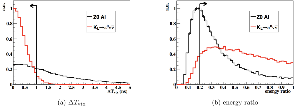
Figure 6.14: Comparison of the \Delta T_{\text{vtx}} (left) and energy ratio (right) distributions between the Z0 AI data (the hadron-cluster events) and the K_L \rightarrow \pi^0 \nu \bar{\nu} signal MC. The black lines and arrows indicate the region accepted by the cuts.
