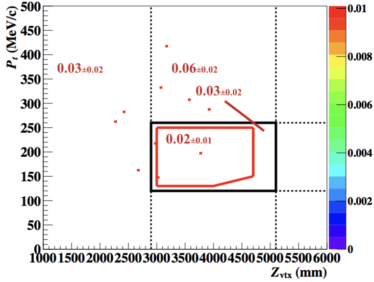
Figure 6.42: P_t - Z_{\text{vtx}} distribution of the K_L \rightarrow 2\gamma background events. Numbers in red indicate the number of events in each region bounded by lines.
