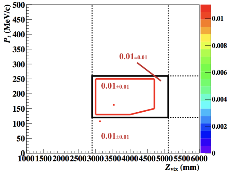
Figure 6.43: P_t - Z_{\text{vtx}} distribution of the K_L \rightarrow 3\pi^0 background events. Numbers in red indicate the number of events in each region bounded by lines.
