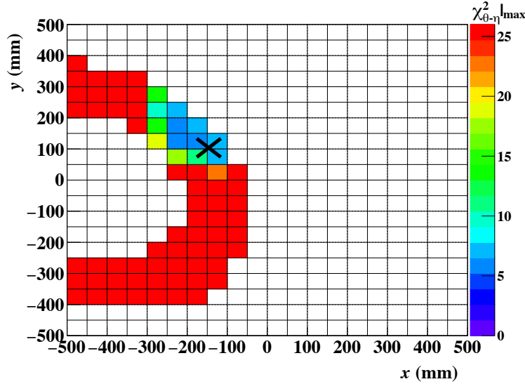
Figure 6.55: \chi^2_{\theta-\eta}|_{\text{max}} distributions of a CV- \eta event. The colored region represents the \eta vertex candidates. The black cross mark indicates decay position of \eta obtained from simulation record.
