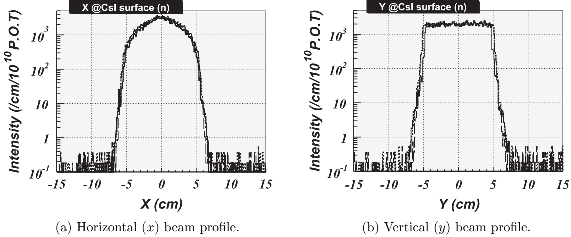
Figure 2.9: Neutron profile at the surface of the CsI calorimeter (quoted from Ref. [54]).
