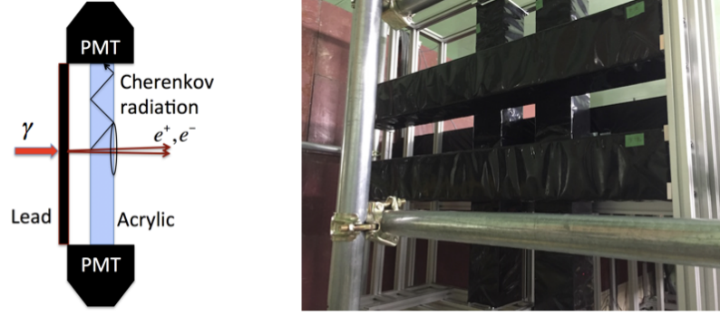
Figure 2.27: Left: Schematic view of a BHGC module (quoted from Ref. [73]). Right: a picture of BHGC viewed from downstream (quoted from Ref. [74]).
