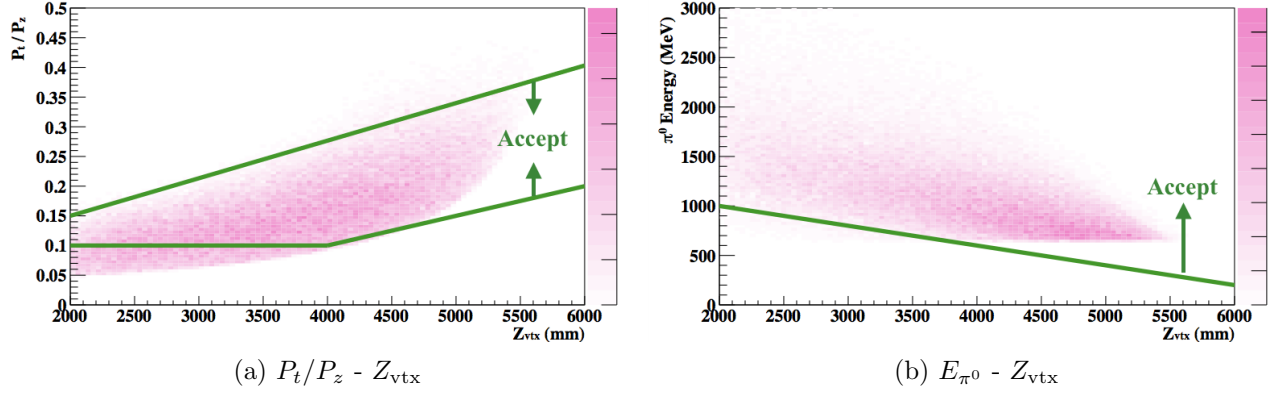
Figure 6.15: P_t/P_z - Z_{\text{vtx}} and E - Z_{\text{vtx}} selection. Distribution of the K_L \rightarrow \pi^0 \nu \bar{\nu} events is shown with the accepted region bounded by green lines.
