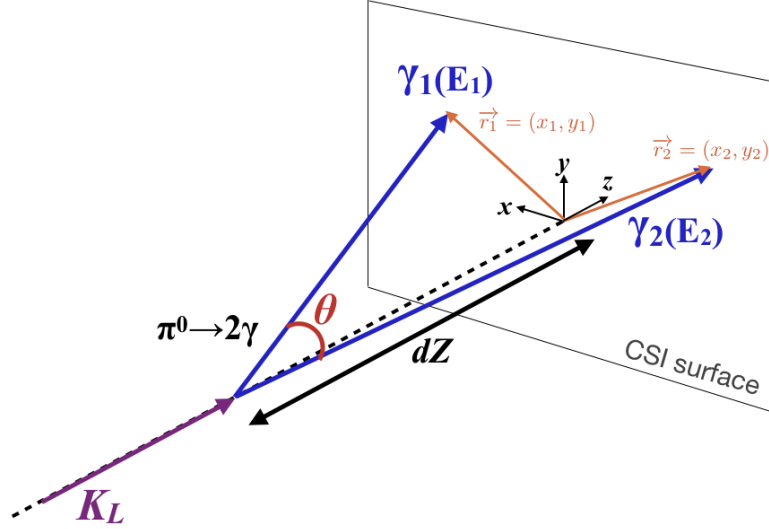
Figure 4.8: Reconstruction of the \pi^0 \rightarrow 2\gamma decay with the CsI calorimeter.
