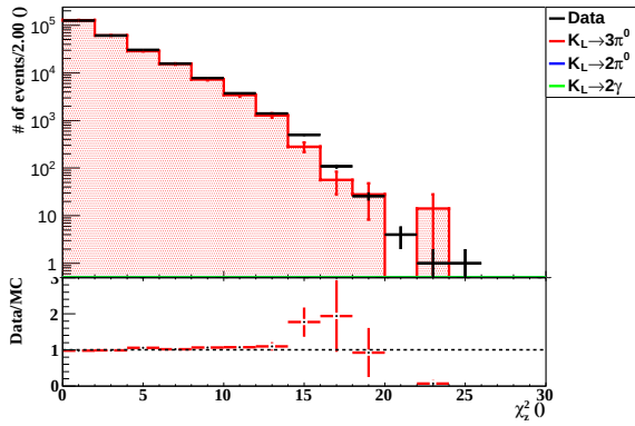
(e) \chi^2_0
