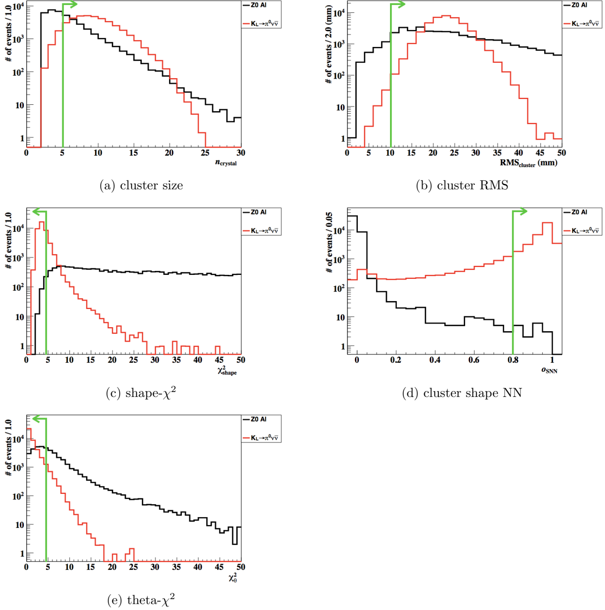
Figure 6.18: Distributions of variables used for the shape-related cuts under a loose cut condition. Z_{\text{vtx}} > 2900 \text{ mm} is required to eliminate the contribution from the upstream- \pi^0 events. The black histograms represent the hadron-cluster control sample taken in the Z0 AI run and the red histograms represent the K_L \rightarrow \pi^0 \nu \bar{\nu} MC. The green lines and arrows indicate the region accepted by the cuts.
