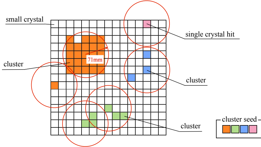
Figure 4.5: Example of the grouping of cluster seeds (quoted from Ref. [57]). Each box represents a small crystal and colored one denotes a cluster seed. The cluster seeds with the same color belong to the same cluster. The red circles with a radius of 71 mm represent the grouping region. There are three clusters (orange, green, blue) and one isolated hit crystal (magenta) in this figure.
