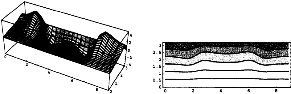
Figure 8. Shape of \Upsilon_N and contour field of \delta T(1 - z/\pi - \Upsilon_N/\sqrt{\mathcal{R}\mathcal{P}}\pi) + T(T = 0, \delta T = 5)
