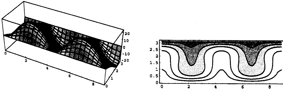
Figure 6. Shape of \Theta_N and contour field of
