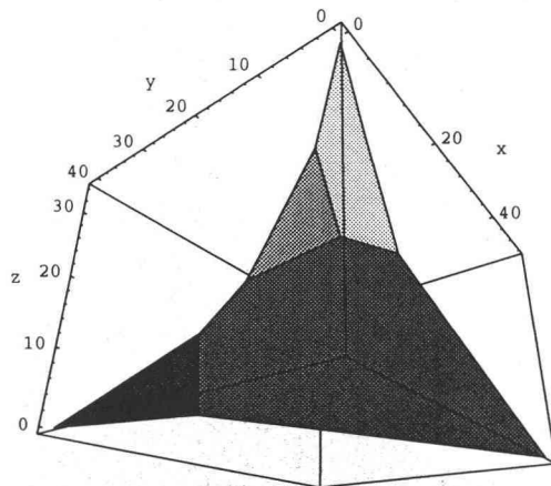
FIGURE 4. C_\zeta for \frac{1}{5}(1, 2, 3) , \zeta = (9, 8, -3, -2, -12) , giving a smooth resolution.
