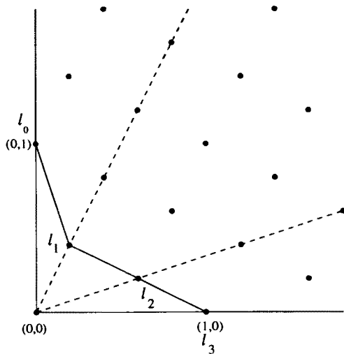
FIGURE 7. The minimal resolution of \frac{1}{5}(1, 2) constructed by toric means.
