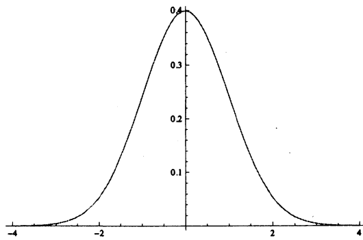
Figure 1: Probability density of the standard Gaussian g
