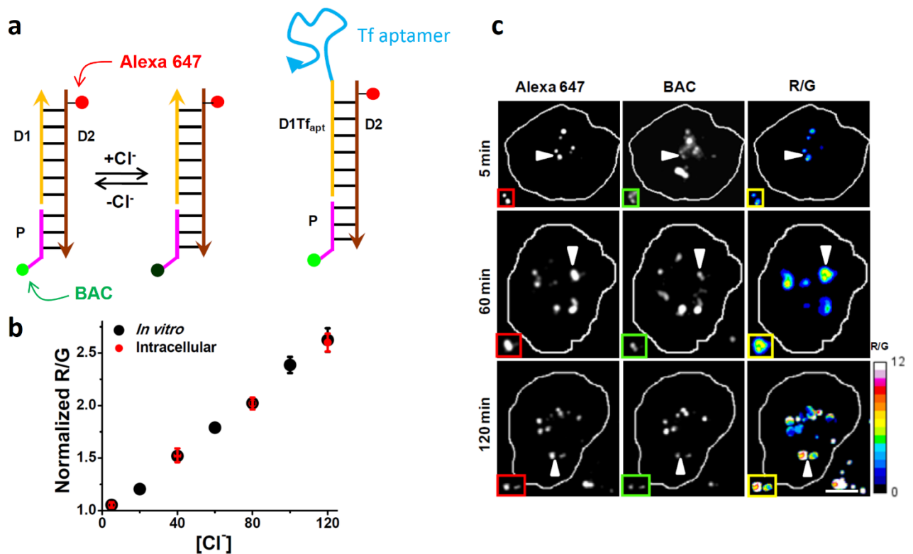
Figure 1: Clensor functions in the subcellular components.
