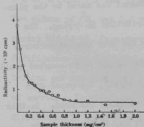
Fig. 5 Self-absorption of Inositol- ^3\text{H} . Inositol- ^3\text{H} containing different amounts of carrier was pipetted onto stainless planchet (diameter 25 mm), and after drying radioactivity was determined.
