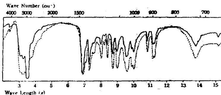
Fig. 1 Infrared Spectrum of myo -Inositol and myo -Inositol- ^3\text{H} , Labeled by Recoil Triton Method. (Nujol mull) : myo -Inositol — : myo -Inositol- ^3\text{H}
