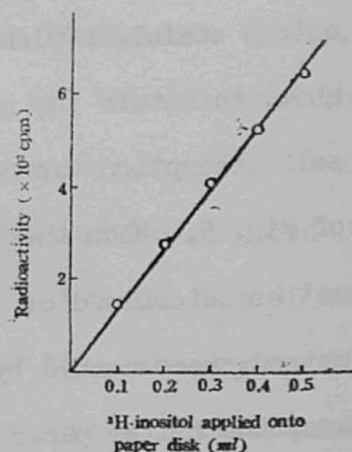
Fig. 6 Radioactivity of Inositol- ^3\text{H} Measured by Paper Disk Method. Different amounts of inositol- ^3\text{H} ( 45.2 \mu\text{g}/\text{cm}^2 per 0.1 ml) was applied onto paper disk, and after drying radioactivity was determined.
