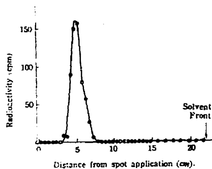
Fig. 2 Distribution of Inositol- ^3\text{H} , Labeled by Recoil Triton Method, on Paperchromatogram. Butanol-Acetic acid-Water, 4:1:5 (upper layer), three multiple developments.
