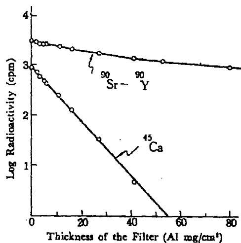
Fig. 1. Absorption of \beta -Rays of ^{45}\text{Ca} and ^{90}\text{Sr}-^{90}\text{Y} by Aluminium. (without correction of air and G.M. tube's mica window thickness)
