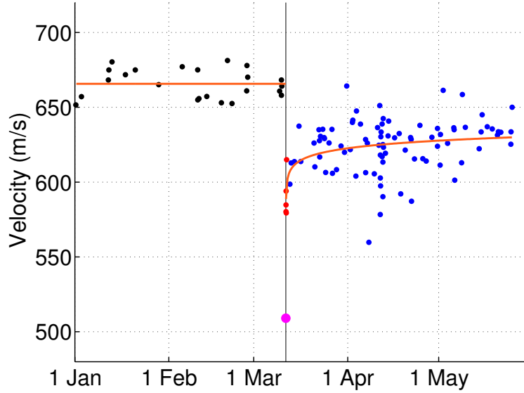
Figure 3. Shear-wave velocity variations in the upper 100 m at station FKSH18. By using the arrival times of waves (the circles in Figure 1), we compute the velocity variations from 1 January 2011 to 26 May 2011. The color of each dot is the same as in Figure 1. Black vertical line indicates the origin time of the Tohoku-Oki earthquake. Orange line depicts the average velocity (before the Tohoku-Oki earthquake) and the logarithm curve determined by least-squares fitting of the velocity after the earthquake. We do not include the Tohoku-Oki earthquake data point (magenta dot) in the data fit.
