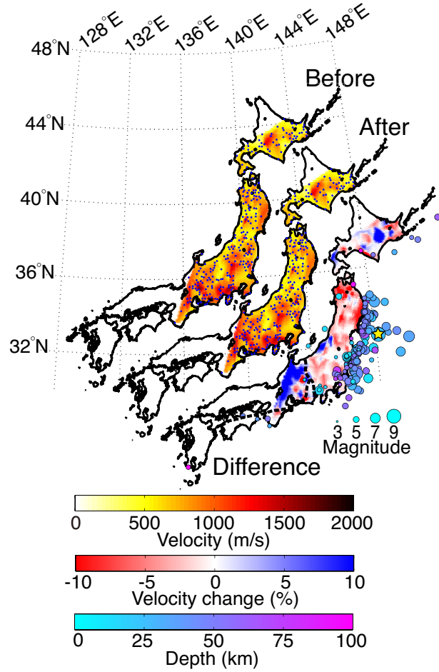
Figure 5. Shear-wave velocities estimated from deconvolved waveforms before (upper-left) and after (middle) the Tohoku-Oki earthquake. Blue dots on these two maps show the KiK-net stations used in this study. The map on the lower-right gives the relative change in shear-wave velocity before and after the event. The longitude and latitude belong to the map in the upper-left. Locations and magnitude of the earthquakes from 1 January 2011 to 26 May 2011 are shown as circles, relative to the map on the lower-right. The size of each circle indicates the magnitude of each earthquake and the color represents the depth. The yellow star denotes the location of the Tohoku-Oki earthquake. The dashed black lines show the locations of MTL and ISTL [Ito et al. , 1996].
