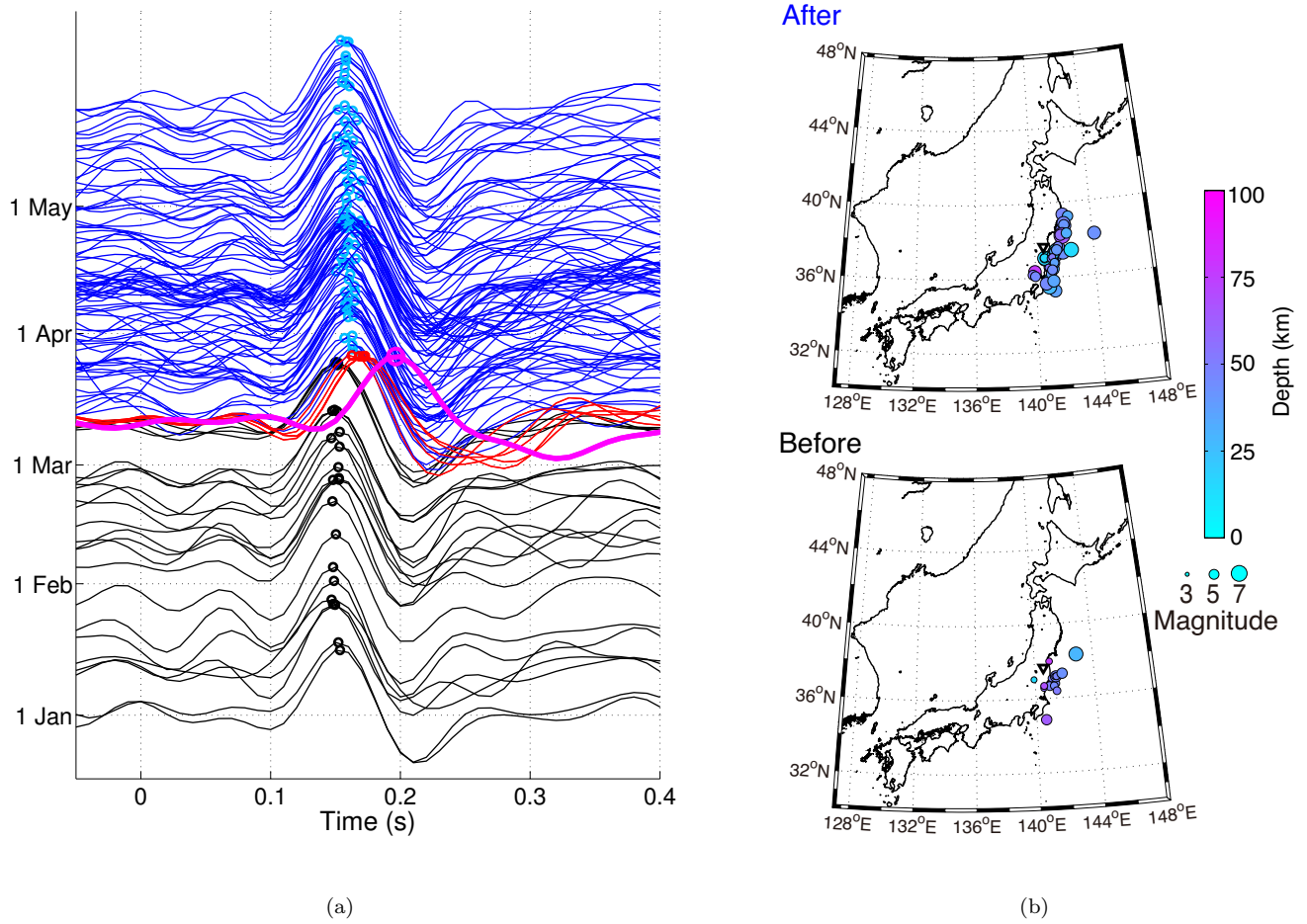
Figure 1. (a) Deconvolved waveforms of individual earthquakes from 1 January 2011 to 26 May 2011 at station FKSH18. This station recorded 25 earthquakes from 1 January 2011 to 10 March 2011 (black curves), the Tohoku-Oki earthquake of 11 March 2011 (magenta thick curve), 5 other earthquakes on 11 March 2011 (red curves), and 96 earthquakes from 12 March 2011 to 26 May 2011 (blue curves). Circles, marked by the same color as the waveforms (blue replaces cyan), represent the interpolated arrival times of waves. The waveforms are ordered by the origin times of earthquakes in the vertical axis. (b) Epicenters of two time intervals: 1 January 2011 to 10 March 2011 and 12 March 2011 to 26 May 2011. The size of each circle indicates the magnitude of each earthquake and the color denotes the depth. The white triangle points to the location of station FKSH18.
