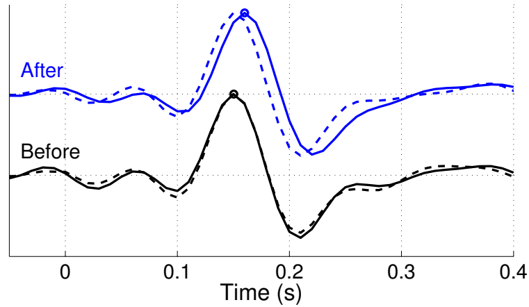
Figure 4. Averaged waveforms of Figure 1 before (from 1 January 2011 to 10 March 2011; black solid curve) and after (from 12 March 2011 to 26 May 2011; blue solid curve) the Tohoku-Oki earthquake at station FKSH18. Circles denote the interpolated arrival times of averaged waves. Black and blue dashed curves represent the averaged waveforms from 1 January to 10 March and from 12 March to 26 May over 11 years (from 2000 to 2010), respectively.
