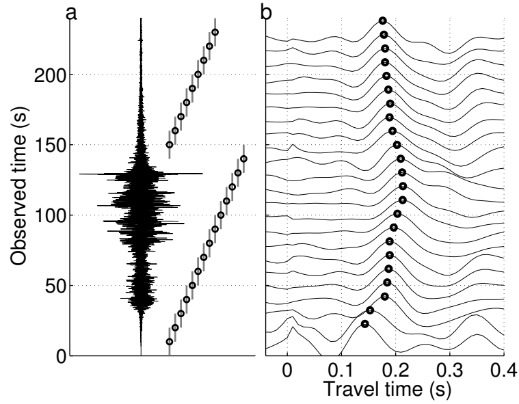
Figure 2. Short-time moving-window seismic interferometry of the ground motion caused by the Tohoku-Oki earthquake. (a) The earthquake record observed at the north-south horizontal component borehole seismometer of station FKSH18. Gray bars indicate the 20-s time windows for seismic interferometry with 10-s overlap. Black circles are the center of each window. (b) Deconvolved waveforms of each time window. Each waveform is aligned with the center time of the employed time window. Black circles illustrate the interpolated arrival times.
