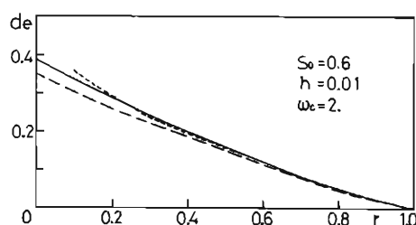
(b) Equivalent damping coefficient.
