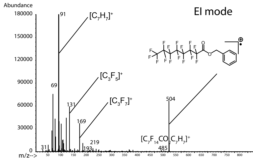
Fig. 1 Mass spectra of PFOA benzyl ester in EI mode and ECNI mode (m/z 30–800)
