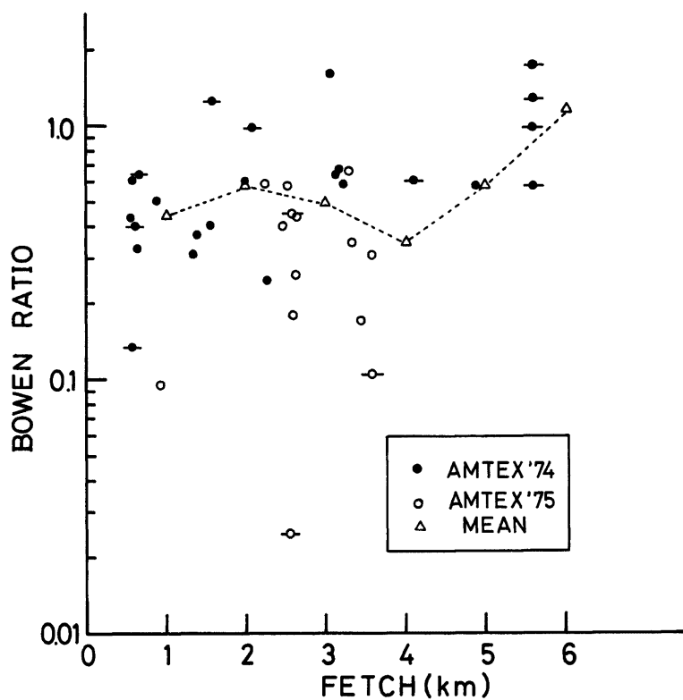
Fig. 11. The Bowen ratio as a function of fetch. The horizontal bar denotes the data of small fluxes (less than 1 mW/cm 2 ).
