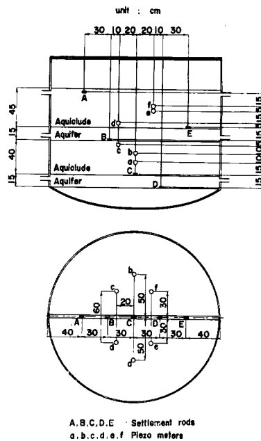
Fig. 3 Soil profile and position of measuring apparatus.
