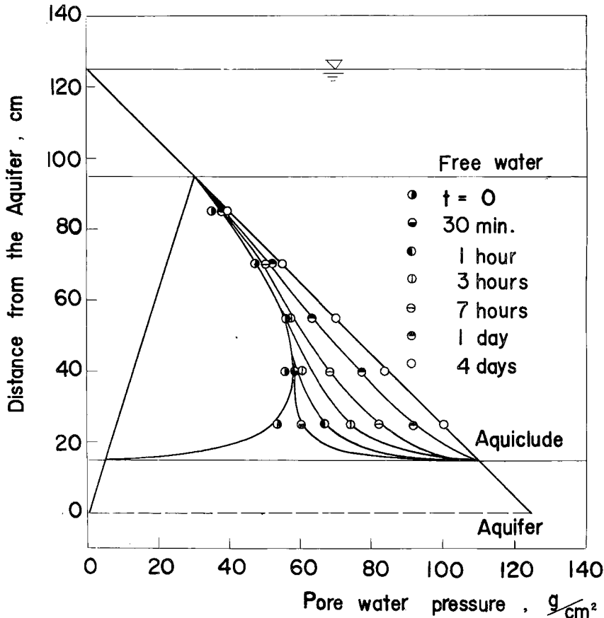
Fig. 11 Measured results of pore water pressure after the artesian head in the aquifer was recovered.
