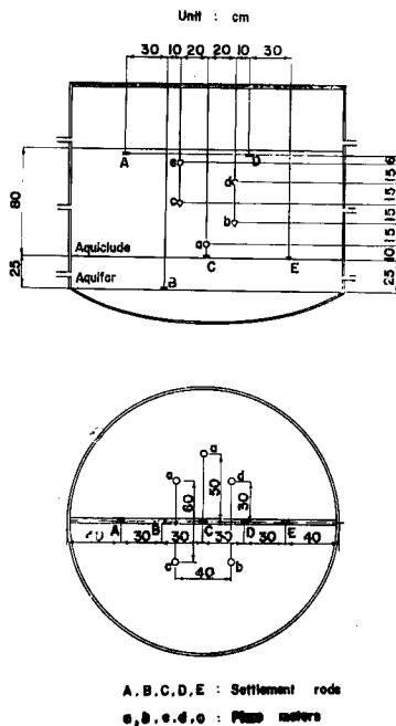
Fig. 2 Soil profile and position of measuring apparatus.
