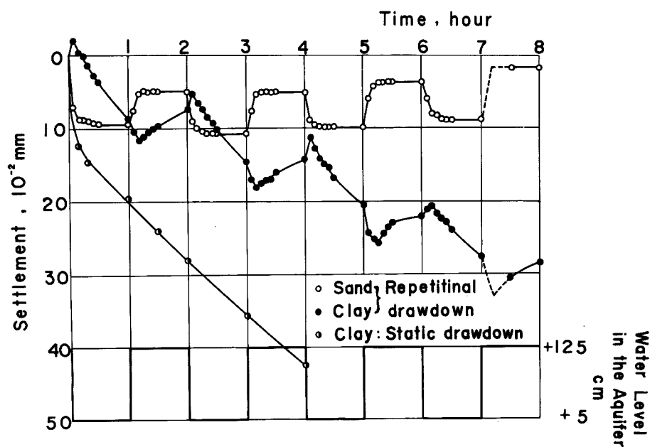
Fig. 15 Behavior of the subsidence due to repetitional drawdown of the artesian head.
