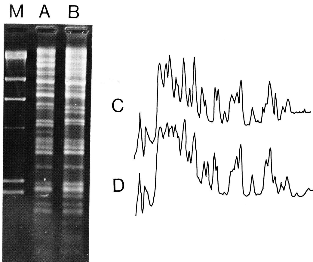
Fig. I-2. Electrophoresis on a 0.7% agarose gel of rice mitochondrial DNA digested with Pst I. Mitochondrial DNAs were isolated from normal (A) and cms-Bo cytoplasms (B). Lane M shows molecular weight marker; lambda DNA digested with Hind III. Negative film obtained in this experiment was scanned with a densitometer. Panels C and D represent profiles of the pattern of DNA restriction fragments from lanes A, B respectively. The top of the gel is on the left hand side. One peak of this figure represents one DNA fragment. The concentration of the DNA fragment reflects the area of peak.
