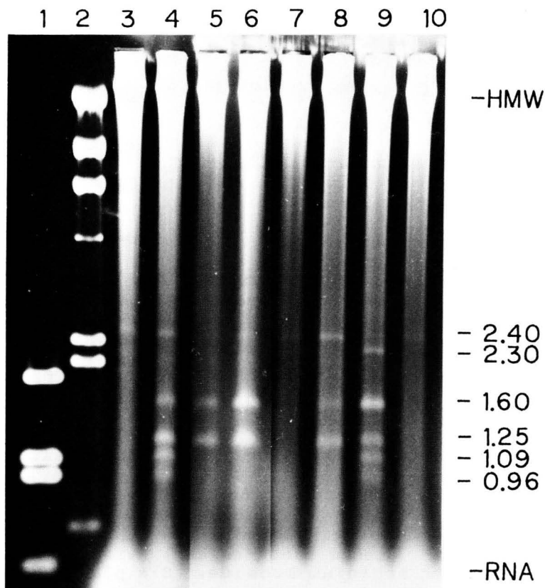
Fig. III-1. Distribution and variation of the mitochondrial plasmid-like DNAs in rice cultivars. Mitochondrial DNAs isolated from etiolated rice seedlings were incubated with RNase A and separated by electrophoresis on 0.7% agarose gel without restriction enzyme treatment.
