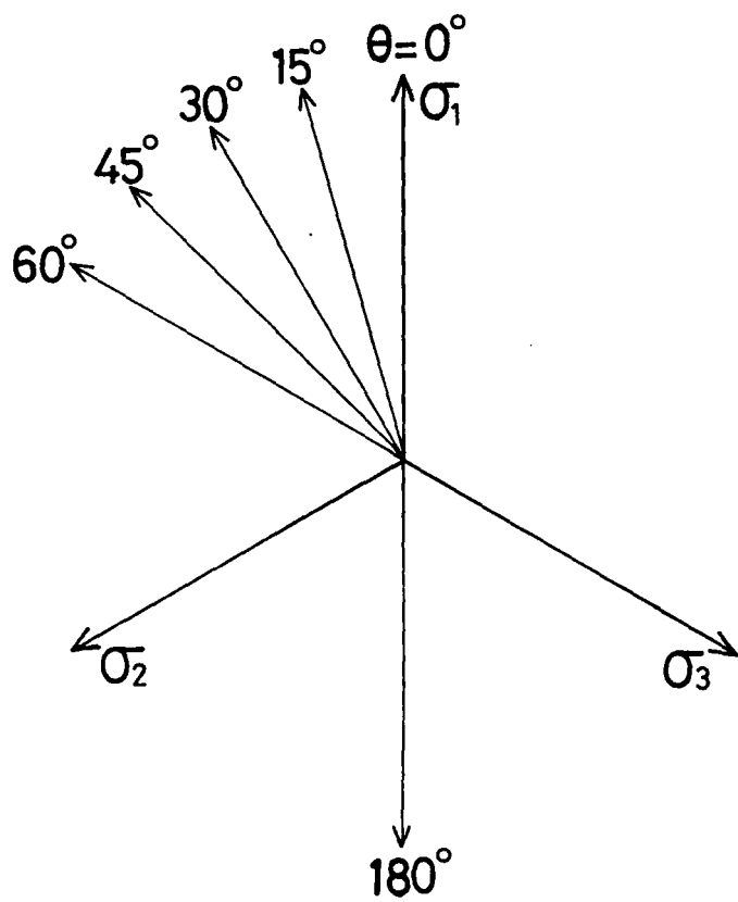
Fig.5.5 Stress paths on \pi -plane
