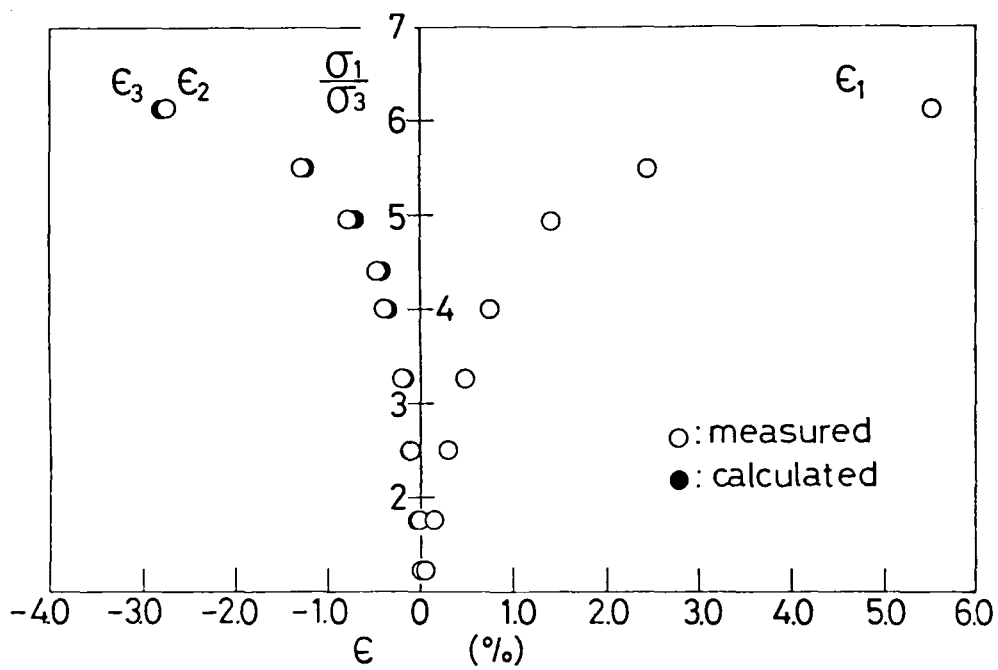
Fig.5.9 Measured and calculated strains under axis-symmetric stress state
