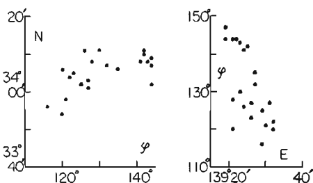
Fig. 12 Relation between the direction of the pressure and the location of the origin of the Miyake-jima Swarm.
