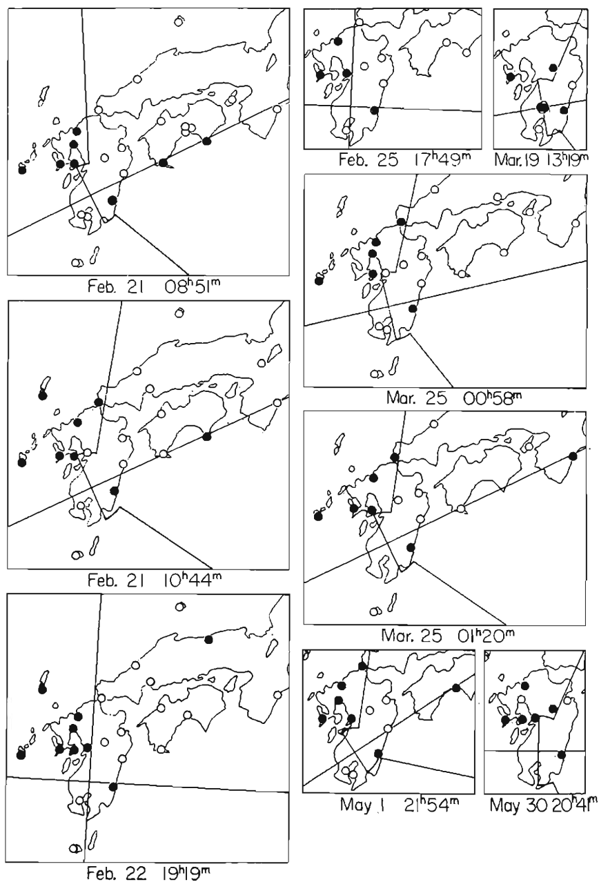
Fig. 10 Nodal lines of the major shocks of the Ebino Swarm.
