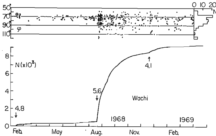
Fig. 5 Direction of the pressure (after Watanabe et al.).
