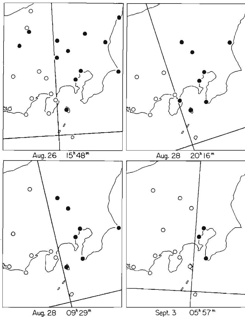
Fig. 11 Examples of the Push-pull distributions of the Miyake-jima Swarm.
