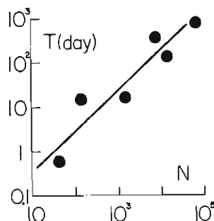
Fig. 3 Relation between the total number and the duration time.
