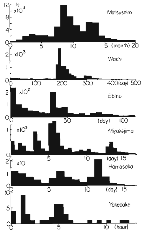
Fig. 2 Time variation of the number of shocks.
