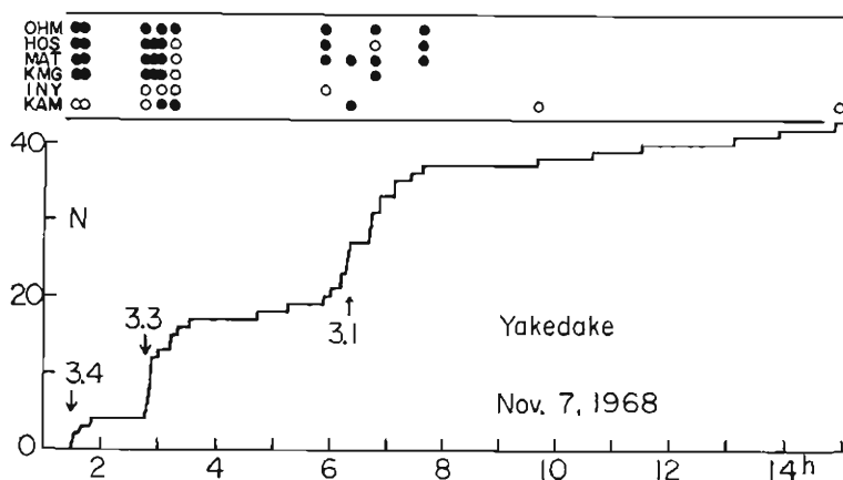
Fig. 9 Push-pull distribution and activity.
