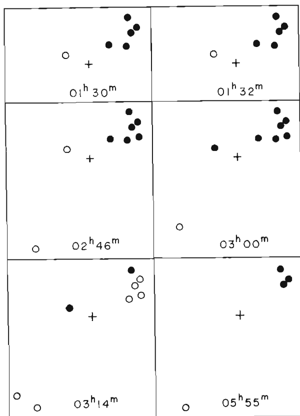
Fig. 15 Push-pull distribution of the major shocks of the Yake-dake Swarm.
