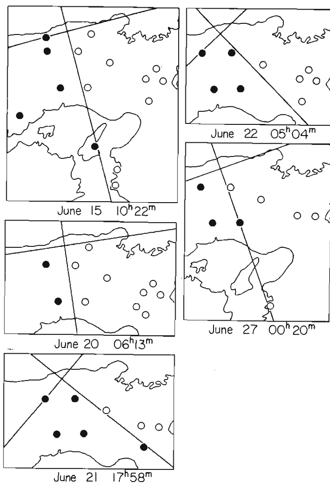
Fig. 13 Nodal lines of the major shocks of the Hamasaka Swarm.
