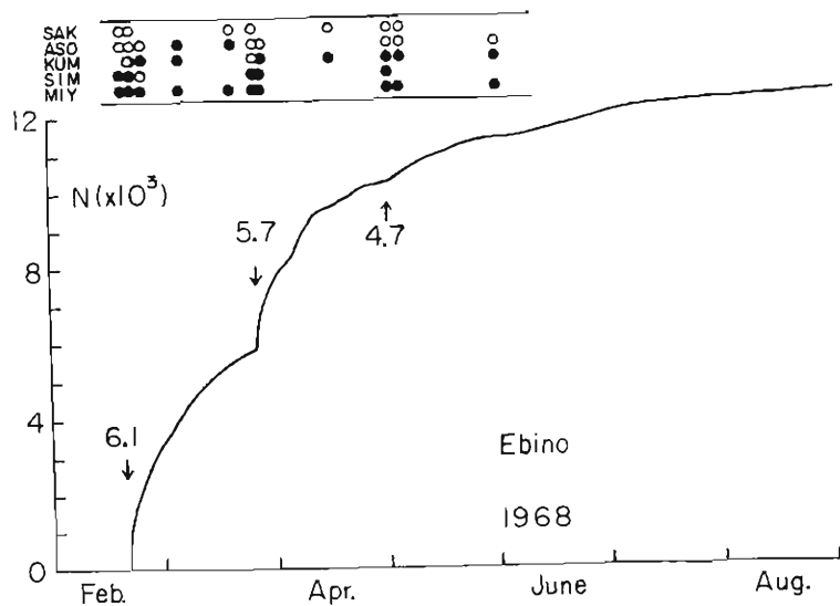
Fig. 6 Push-pull distribution of the first P motions and activity.
