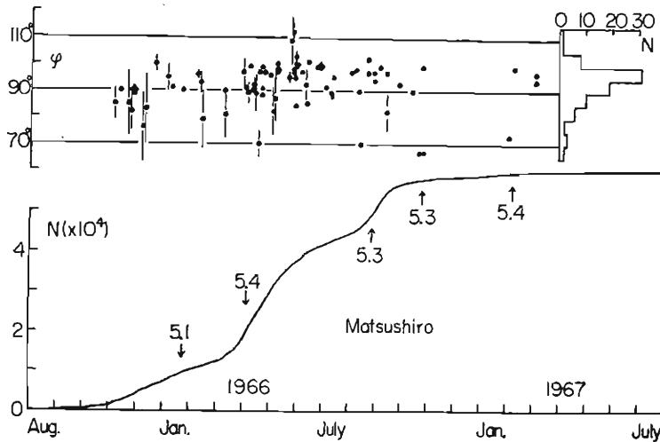
Fig. 4 Direction of the pressure (after Ichikawa) and activity.
