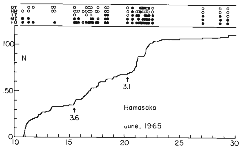
Fig. 8 Push-pull distribution and activity.
