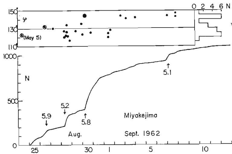
Fig. 7 Direction of the pressure and activity.
