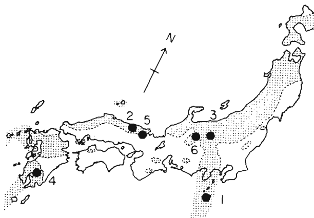
Fig. 1 Dotted area indicates the volcanic region. Numbers correspond to those in Table 1.
