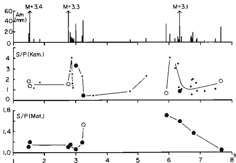
Fig. 14 Time variation of S/P of the shocks of the Yake-dake Swarm observed at Kamitakara and Matsushiro.
