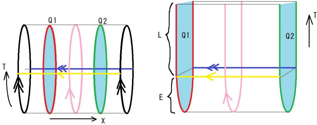
Figure 34. The picture of the dual geometry in the BTZ phase. The left figure describes Euclidean geometry, and the right figure describes Lorentzian time evolution. In this case we impose the dual boundary surface has two connected components Q_1, Q_2 .
