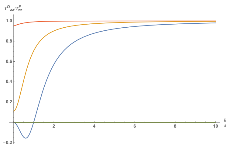
Figure 48. Plots of the ratio (6.53). We used h_L = 2 and \alpha = 0.7 and h_H = 10 .
