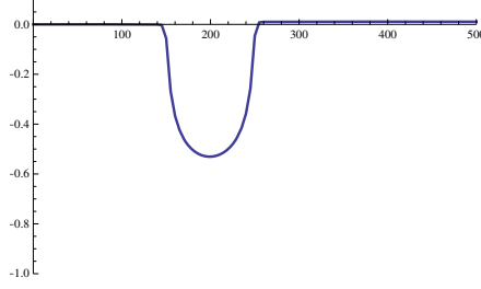
Figure 42. The ratio \Delta S_A^D - (\Delta S_A^{S(x=b)} + \Delta S_A^{S(x=-b)}) under the time evolutions of EE in the splitting quenches of Dirac fermion CFT. We chose the subsystem (i) and set a = 2 and b = 50 .
