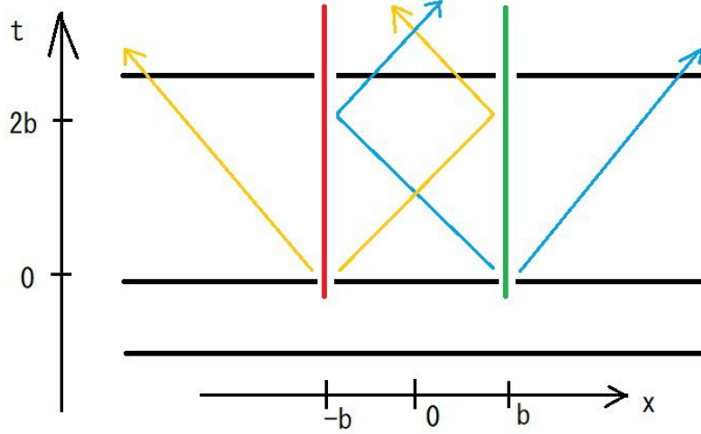
Figure 39. Sketch of a quasi-particle picture. Since single quench creates two quasi-particles, double splitting quench creates four quasi-particles, which is described by blue and yellow lines. These particles move at light speed. Two particles go away from quench point and the other two are trapped in the interval [-b, b] .
