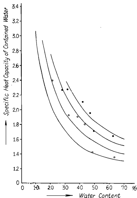
Fig. 2.15 Specific heat capacity of contained water in various water content of remolded and undisturbed clay. (No. 10-27T 27 cm B).
