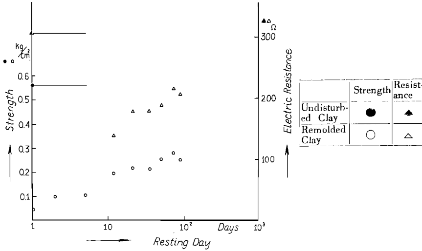
Fig. 2.2. Recovery of strength and of electric resistance
