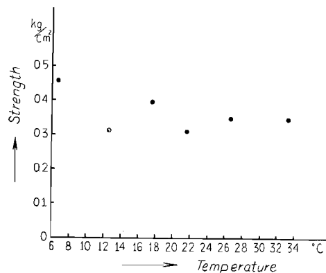
Fig. 2.9 Relation between strength and temperature of remolded clay (Taishobashi 208, 16.16m–17.06m A, Water content 49.5%).
