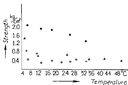
Fig. 2.16 Relation between strength and temperature.
