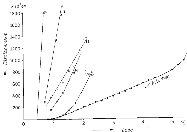
Fig. 2.1 Stress-strain relation in stress control test (6A6-5, 916-S) Figures in the diagram indicate resting days.
