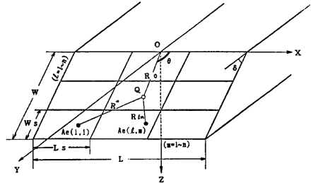
Fig. 3 Fault model
