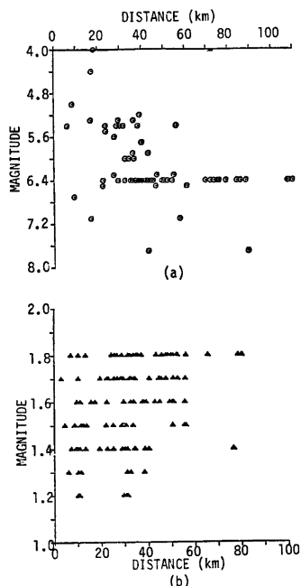
Fig.1 Relation of the magnitudes and the epicentral distances
