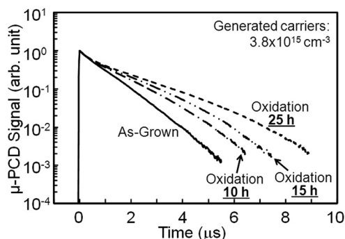
FIG. 3. \mu -PCD decay curves for a 147- \mu m thick p-type 4H-SiC epilayer after oxidation at 1350 °C for 10, 15, and 25 h.
