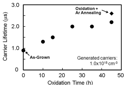
FIG. 4. Oxidation-time dependence of carrier lifetime for a 147- \mu m thick p-type 4H-SiC epilayer with various oxidation times up to 45 h.
