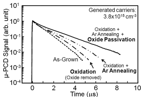
FIG. 1. \mu -PCD decay curves measured before and after various processing steps (oxidation at 1300 °C for 5 h, Ar annealing at 1550 °C for 30 min, and surface passivation with a nitrided oxide) for a 147- \mu\text{m} thick p-type 4H-SiC epilayer.
