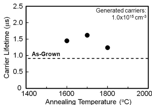
FIG. 5. Annealing temperature dependence of carrier lifetime in 147- \mu m thick p-type 4H-SiC epilayers after carbon implantation process. Carbon ions were implanted at 600 °C to make a 300-nm deep box profile with a carbon concentration of 5 \times 10^{20} \text{ cm}^{-3} .
