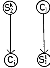
Fig.5-4.4 Subgraphs corresponding to a_2(k,j) \neq 0 and f_1(j,l) \neq 0 .
