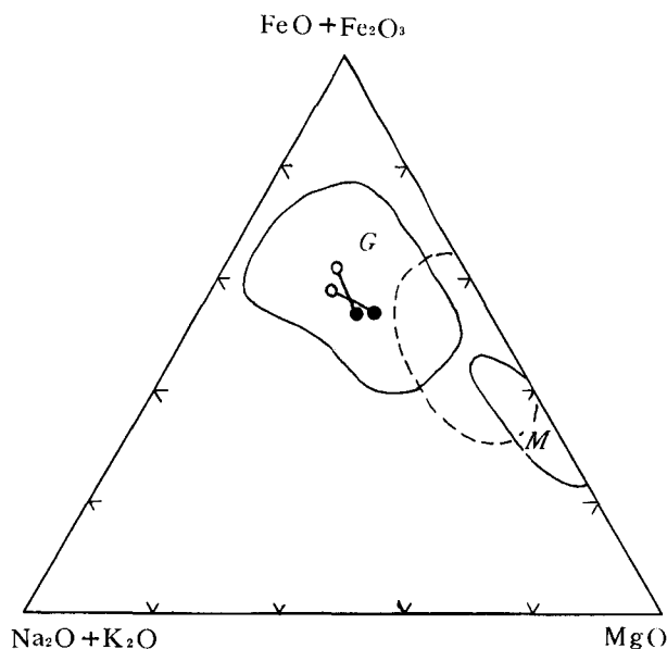
Fig. 7. (\text{FeO} + \text{Fe}_2\text{O}_3) - (\text{Na}_2\text{O} + \text{K}_2\text{O}) - \text{MgO} diagram
