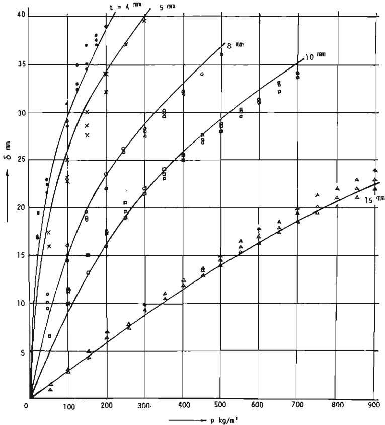
Fig. 4. Comparison of computed deflections with test results; square sheet glass ( t=4 \text{ mm} ) and plate glass ( t=5, 8, 10, 15 \text{ mm} ), size 2000 \times 2000 \text{ mm} .
