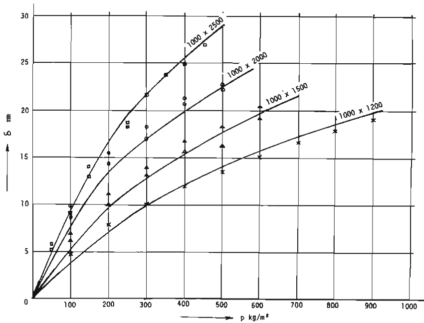
Fig. 6. Comparison of computed deflections with test results; rectangular float glass ( t=6 mm), size 1000 \times 1200 , 1000 \times 1500 , 1000 \times 2000 , 1000 \times 2500 mm.
