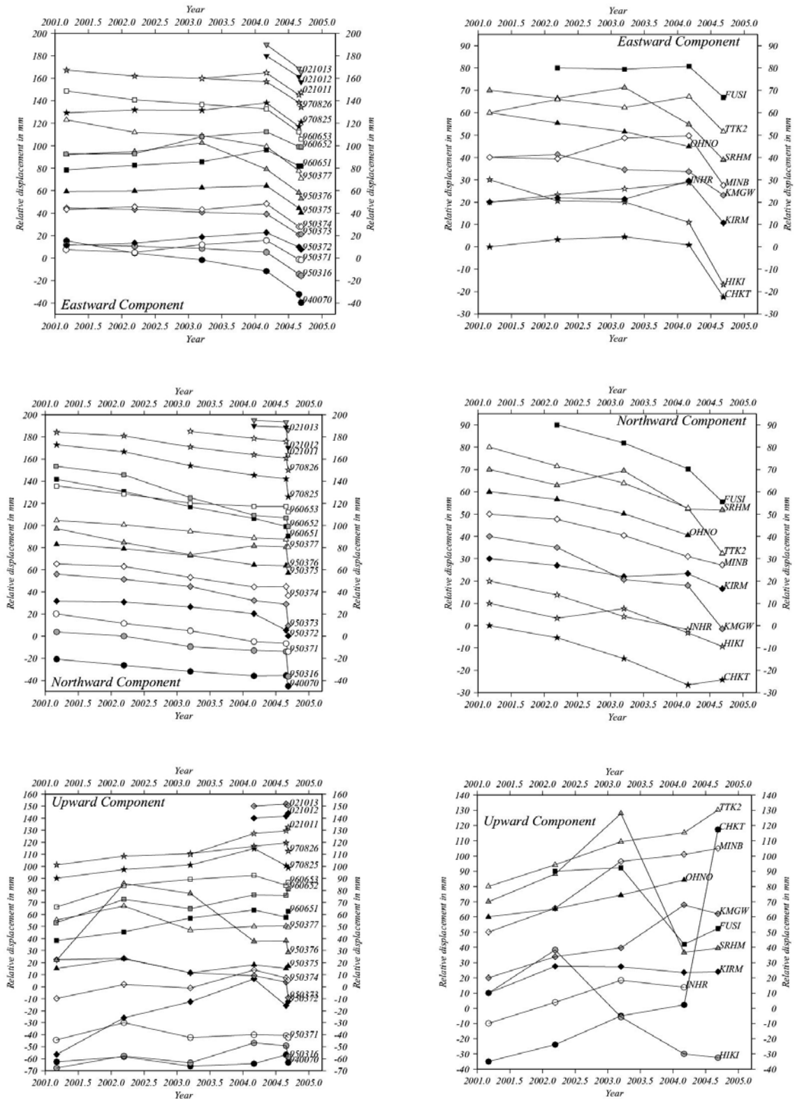
Fig.3 Temporal variations in E-W, N-S and U-D components of site coordinates in ITRF2000 from upper to lower, respectively. Left and right panels show those of GEONET and DPRI sites, respectively.
