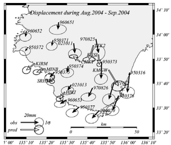
Fig.10 Coseismic displacements of GPS sites relative to the stable Amurian plate derived from DPRI (pred.: white arrows) and GEONET (obs.: black arrows). Those at DPRI sites are estimated by the interpolation of displacement field of GEONET sites
