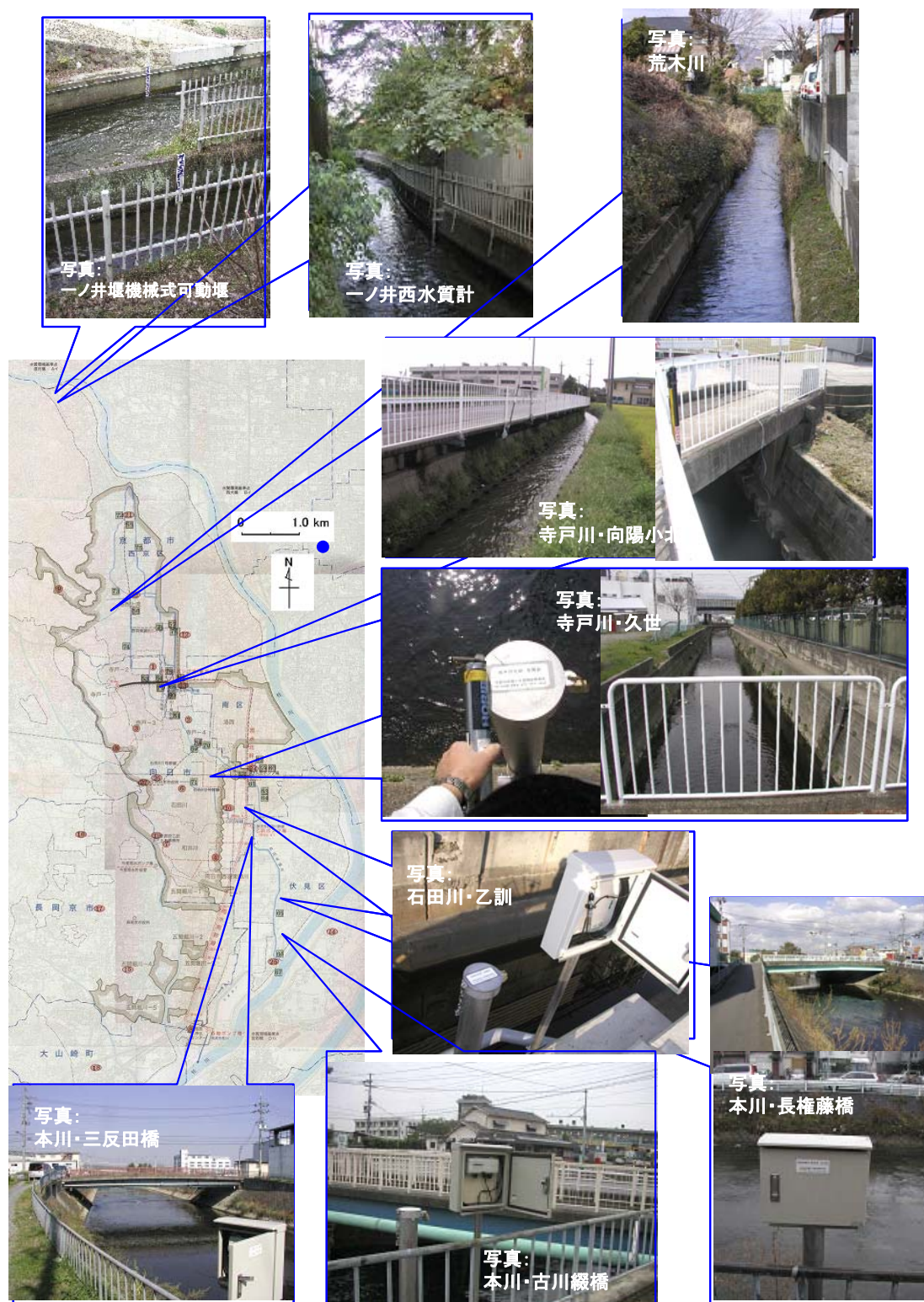
Fig.1 Map of study area and photo of observation stations
