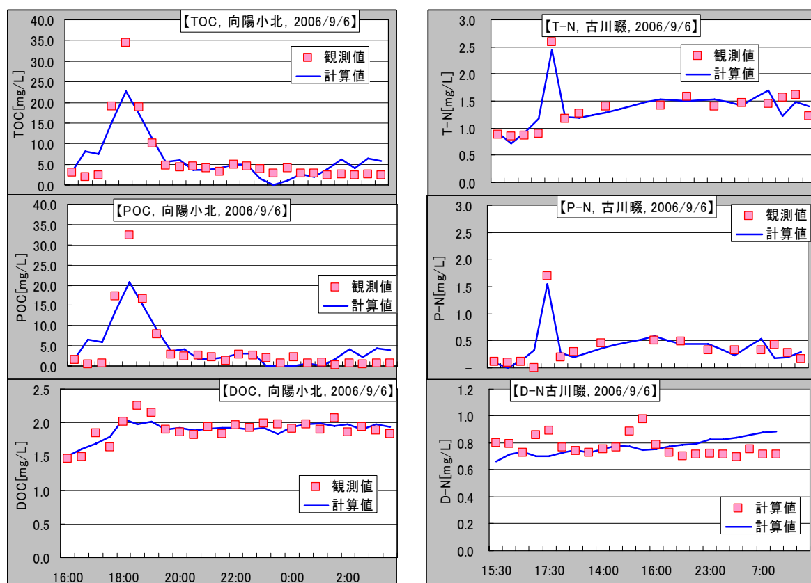
Fig.4 Simulation of pollutant runoff during wet-weather condition
