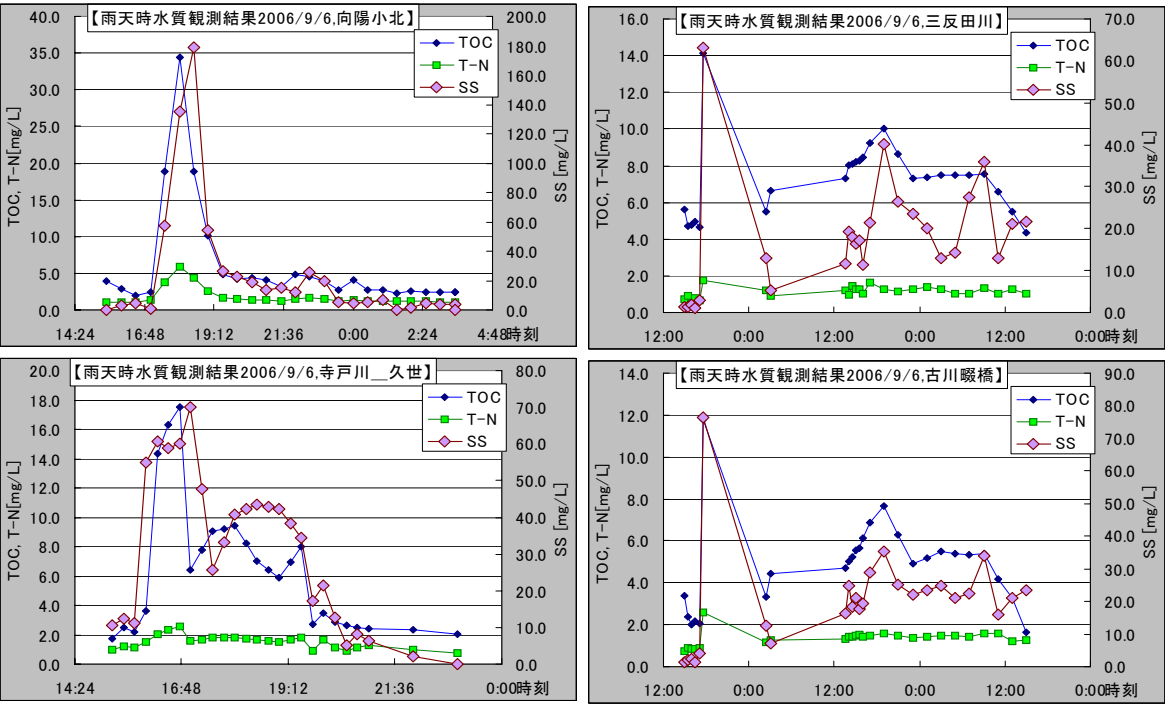
Fig.2 Observed water quality during wet-weather condition in 2006
