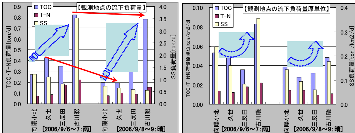
Fig.7 Runoff pollutants load and unit load during flowing down
