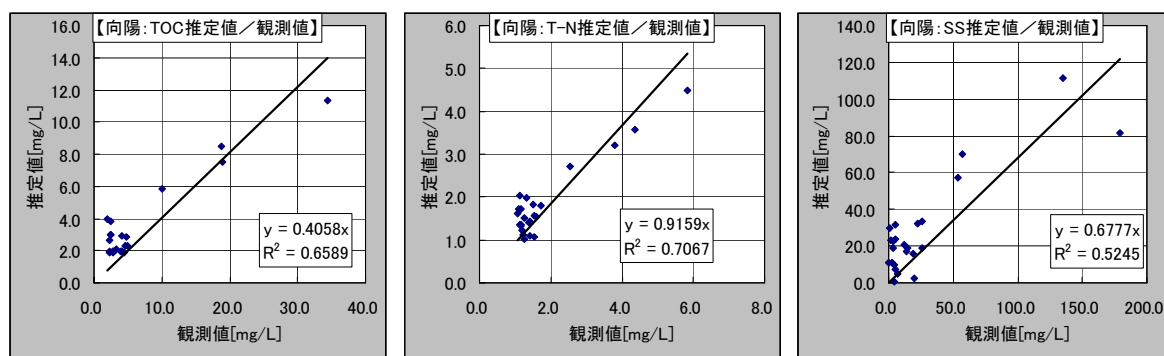
Fig.5 Verification of multi-variable model for water quality
