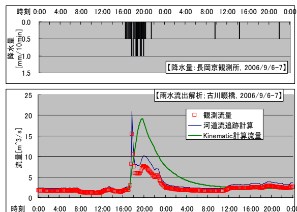
Fig.3 Simulation of stormwater runoff and river water flow during wet-weather condition
