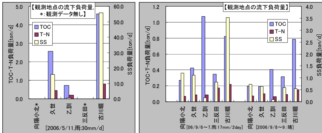
Fig.6 Runoff pollutants load estimated by multi-variable model
