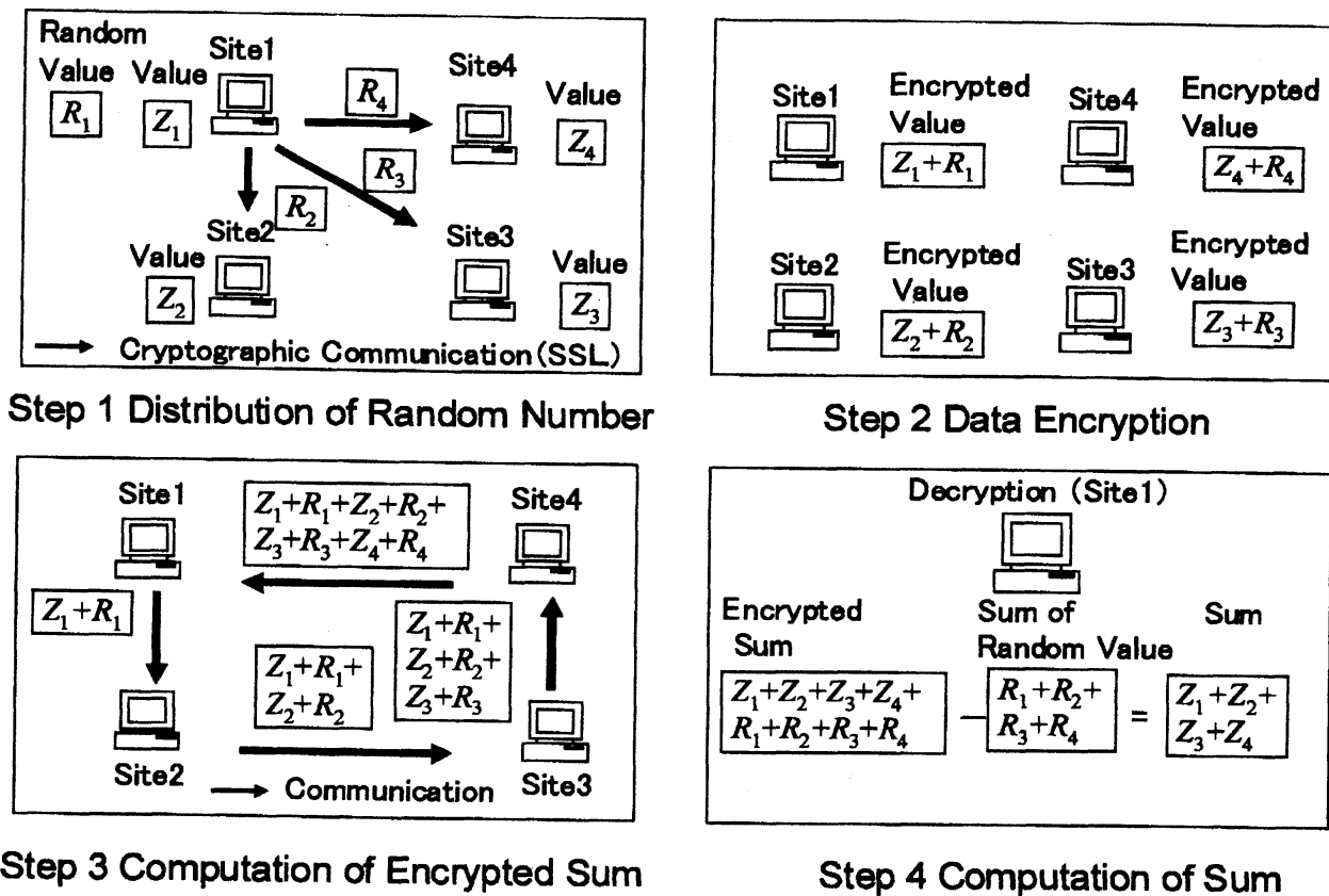
Figure 2: Secure Sum
