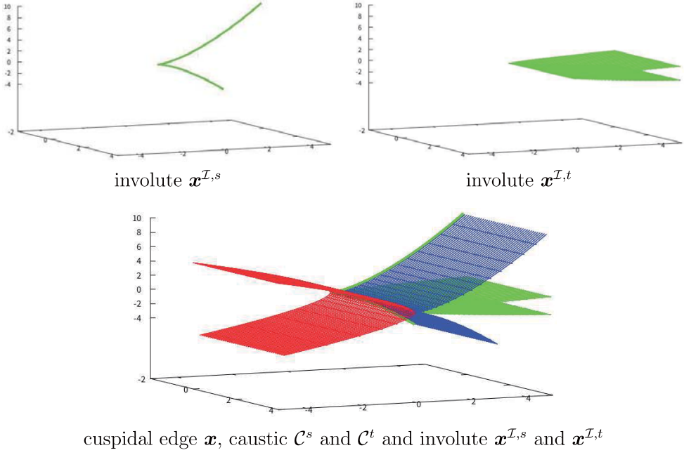
Figures 1 : (\mathbf{x}, \mathbf{n}, \mathbf{s}) and (\bar{\mathbf{x}}, \bar{\mathbf{n}}, \bar{\mathbf{s}}) of Example 6.1
