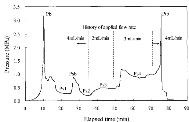
Fig. 10. Pressure history of cyclic pressurize test
