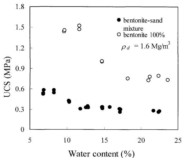
Fig. 4. Unconfined compressive strength (UCS) as a function of water content: The dry density of both materials is 1.6 \text{ Mg/m}^3
