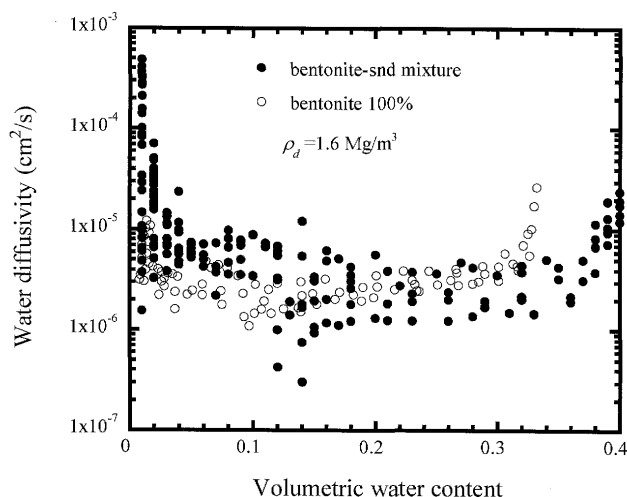
Fig. 2. Water diffusivity as a function of volumetric water content: The dry density of both materials is 1.6 \text{ Mg/m}^3
