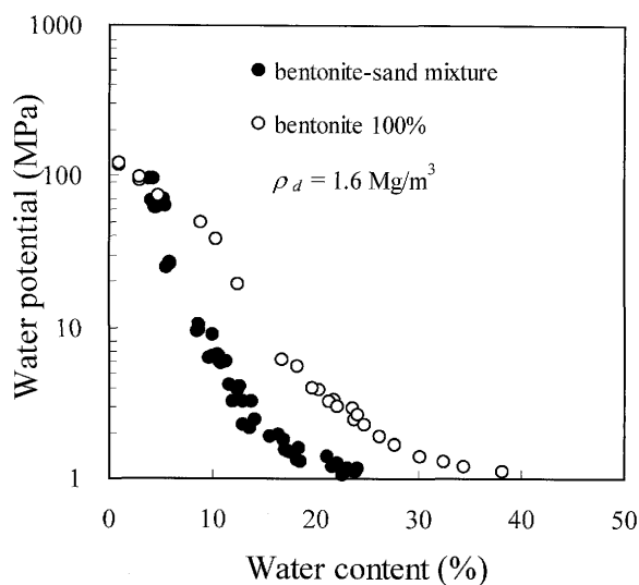
Fig. 3. Water retention curve: The dry density of both materials is 1.6 \text{ Mg/m}^3
