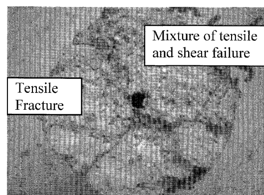
Fig. 9. Example of condition of fracture plane after failure
