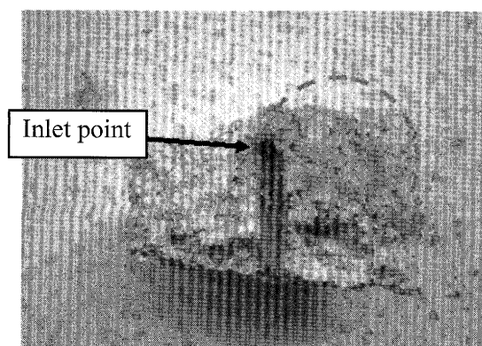
Fig. 9. Example of condition of fracture plane after failure
