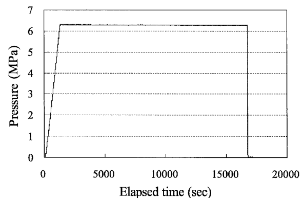
Fig. 12. Pressure history of constant pressure test
