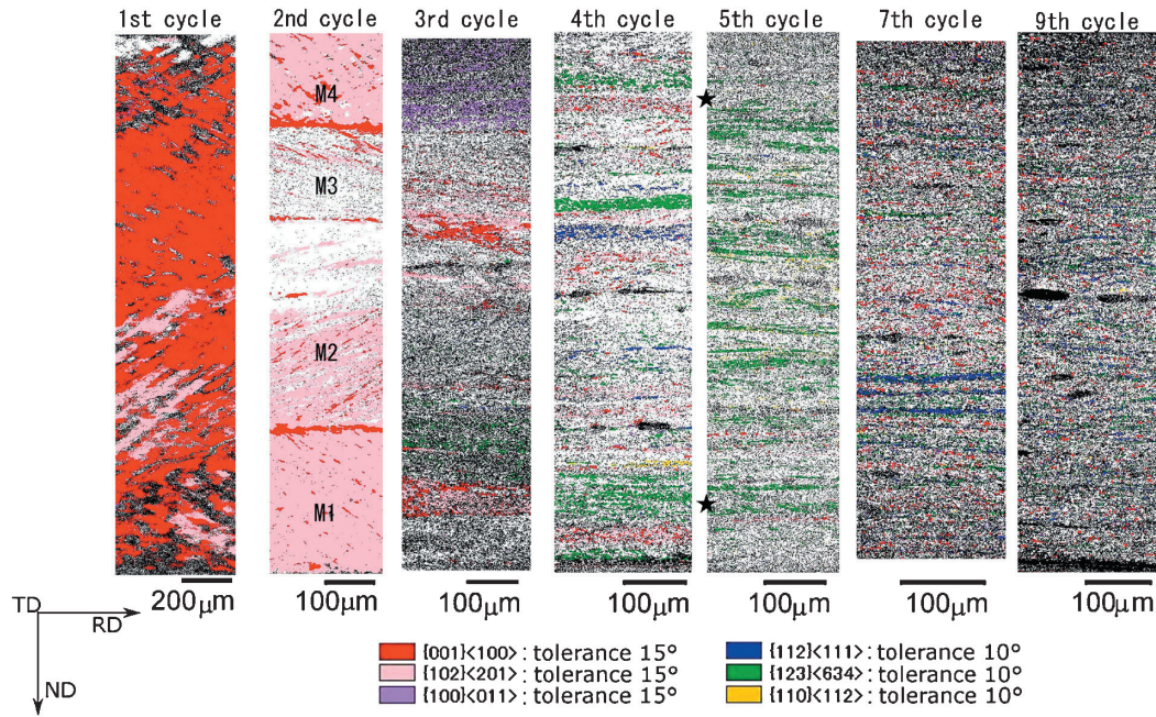
Fig. 5 Crystal orientation maps in processed specimens. These maps show \{100\}\langle 001 \rangle , \{102\}\langle 201 \rangle , and \{100\}\langle 011 \rangle within 15^\circ from the ideal orientations and \{110\}\langle 112 \rangle , \{123\}\langle 634 \rangle , and \{112\}\langle 111 \rangle within 10^\circ from the ideal orientations. The stars indicate one-eighth thickness positions from the surfaces of the 5-cycle processed specimen.
