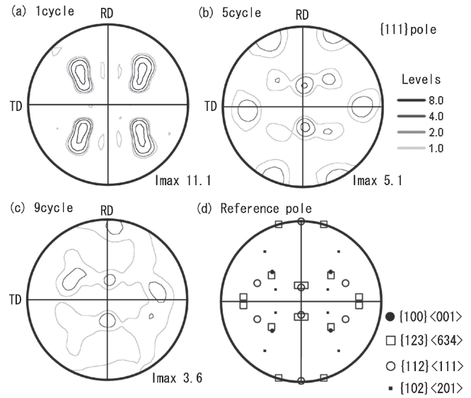
Fig. 2 {111} pole figures of the 1-, 5-, and 9-cycle processed specimens.
