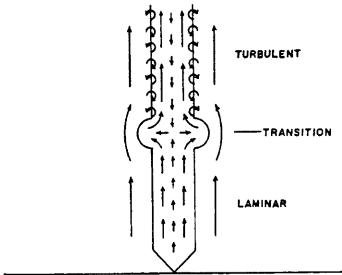
Fig. 13. Schematic representation of the vortex breakdown (after Ward 10) ).
