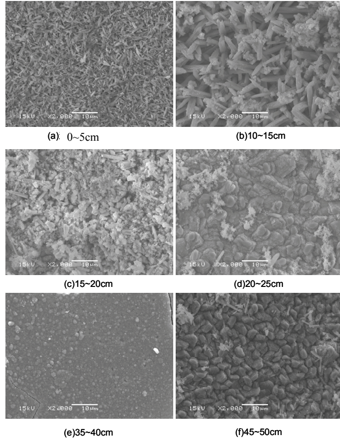
Fig. 3.22: SEM image analysis results at Namikata.
