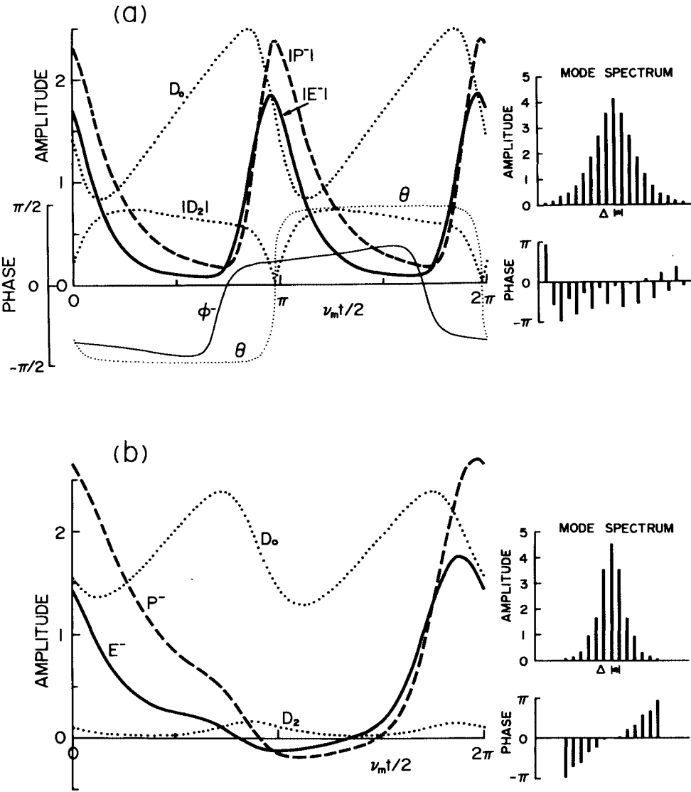
Fig.4.5-7. Two examples of the wave forms at the center of the laser medium for Oscillator A. (a) " \pi -type" locking \delta = -4.0 \times 10^{-3} , (b) "0-type" locking \delta = -12.0 \times 10^{-3} .
