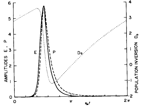
(b) \delta = -0.7 \times 10^{-3}
