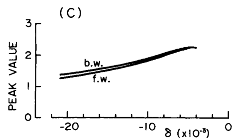
Fig.4.5-4. Pulse peak amplitude and phase shift of the electric field versus detuning.
