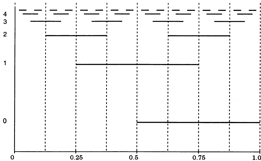
Fig 2: Gray subbase of the unit interval [0,1] . Here, the union of interiors of line segments at level n is G_{n,1} and the interior of the rest is G_{n,0} .
