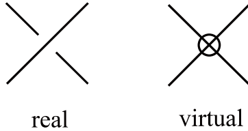
Figure 2: Crossing types.
