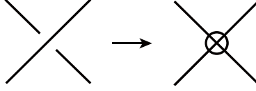
Figure 6: Virtualization.
