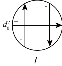
Figure 11: The Gauss diagram I .
