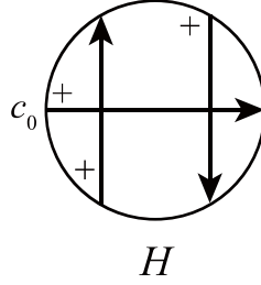
Figure 10: The Gauss diagram H .
