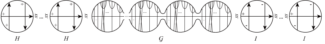
Figure 12: A Gauss diagram \mathcal{G}_m
