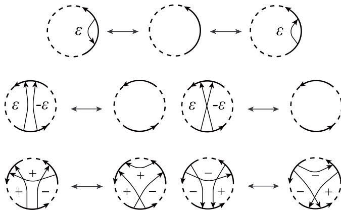
Figure 5: Generalized Reidemeister moves of Gauss diagrams.
