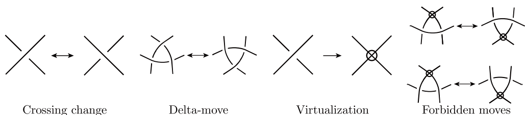
Figure 1: Local moves.
