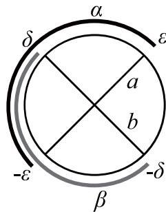
Figure 8: Linked chords a and b .
