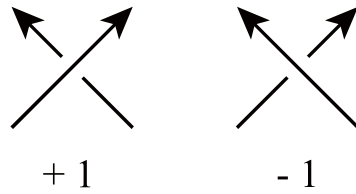
Figure 4: The signs of real crossings.
