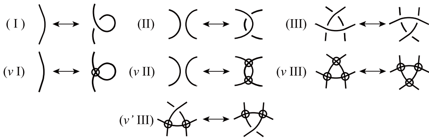
Figure 3: Generalized Reidemeister moves.
