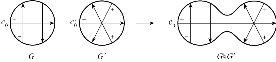
Figure 9: The vertex connected sum G \natural G' .
