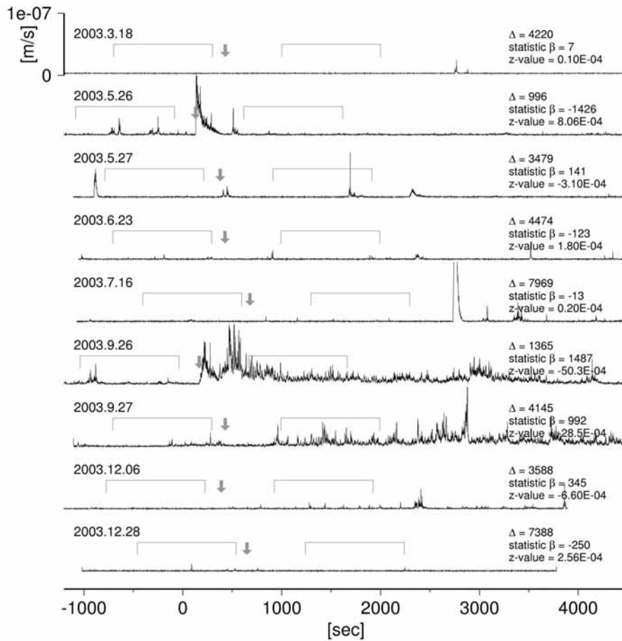
Fig. 9 RMS envelopes constructed from three component waveforms filtered with a pass-band of 5-20 Hz at OZ. Zero indicates the origin time of earthquakes listed in Table 1. Horizontal bars show the 1000 sec time-windows used for calculating the statistic \beta value and z-value. The gray arrows indicate arrival times of the direct P-waves from the corresponding distant earthquake. Vertical scale, velocity, is common. For each event the epicentral distance \Delta , statistic \beta value and z-value are indicated on the right.
