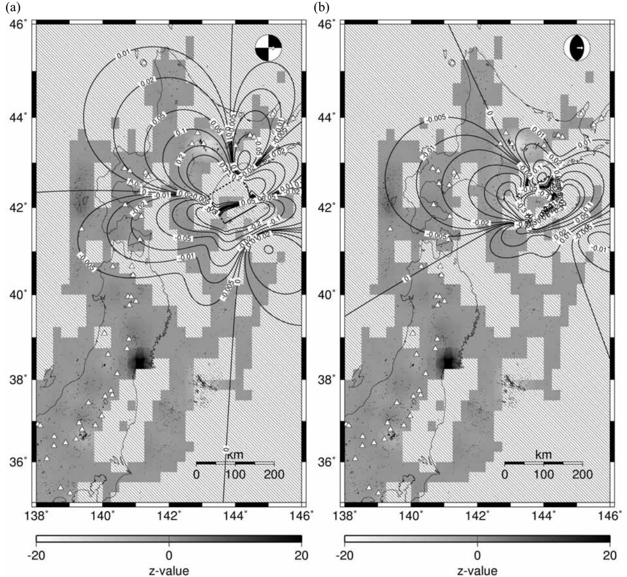
Fig. 3 Z-value and \Delta CFF value. Z-values are estimated from shallow earthquakes (depth \leq 20 km) of magnitude 0 to 5. Rectangular is the fault plane of the 2003 Tokachi-oki earthquake. The pre- and post-seismic periods are Jul 27 to Sep 25 and Sep 26 to Nov 25. Triangles are active volcanoes and dots are the hypocenters of the shallow earthquakes during the post-seismic period. Contour lines in (a) and (b) show the \Delta CFF values in MPa calculated for a depth of 10 km, for two types of faults of the triggered seismicity. The types of faults are (a) EW right lateral and (b) NS strike with eastward dipping (45 deg), as illustrated by the stereoplots in the upper right of each figure. Absolute \Delta CFF values larger than 0.3 MPa are clipped.
