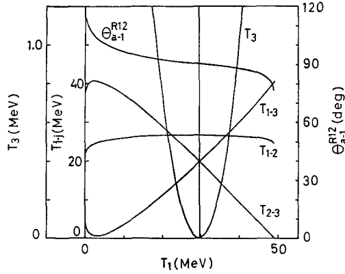
Fig. 1. Kinetic energy T_3 , scattering energy T_{1-2} , scattering angle \theta_{a-1}^{R12} , and relative energies T_{1-3} and T_{2-3} as functions of the kinetic energy T_1 at a coplanar symmetric angle pair \theta_1 = \theta_2 = 41.8^\circ for the {}^3\text{He}(p, pp){}^2\text{H} reaction at 65 MeV.
