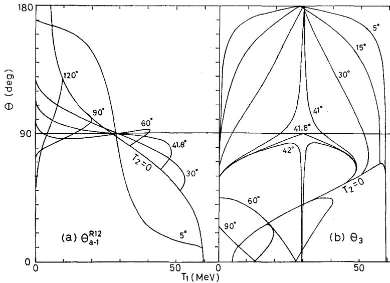
Fig. 5. Scattering angle \theta_{a-1}^{R12} (a) and angle \theta_3 (b) as functions of T_1 , similar to Fig. 3.
