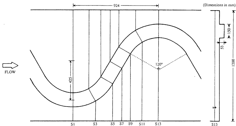
(a) Compound open channel with a meandering main channel (S-M).
