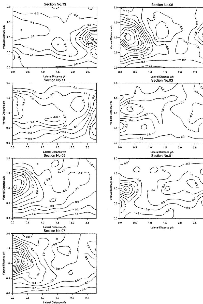
Fig. 8 Reynolds stress -\overline{uw}/u_*^2 for Dr=0.50 . M-M channel.
