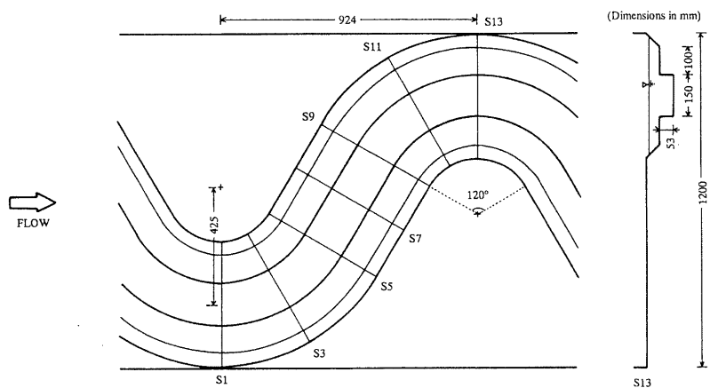
(b) Meandering compound open channel (M-M).
