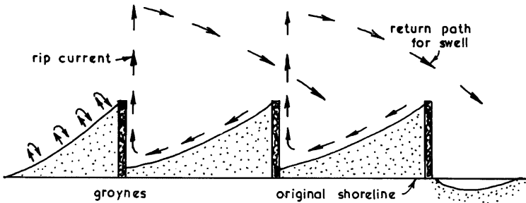
Fig. 2. Path of sediment during storm waves and subsequent swell within a groyne field.
