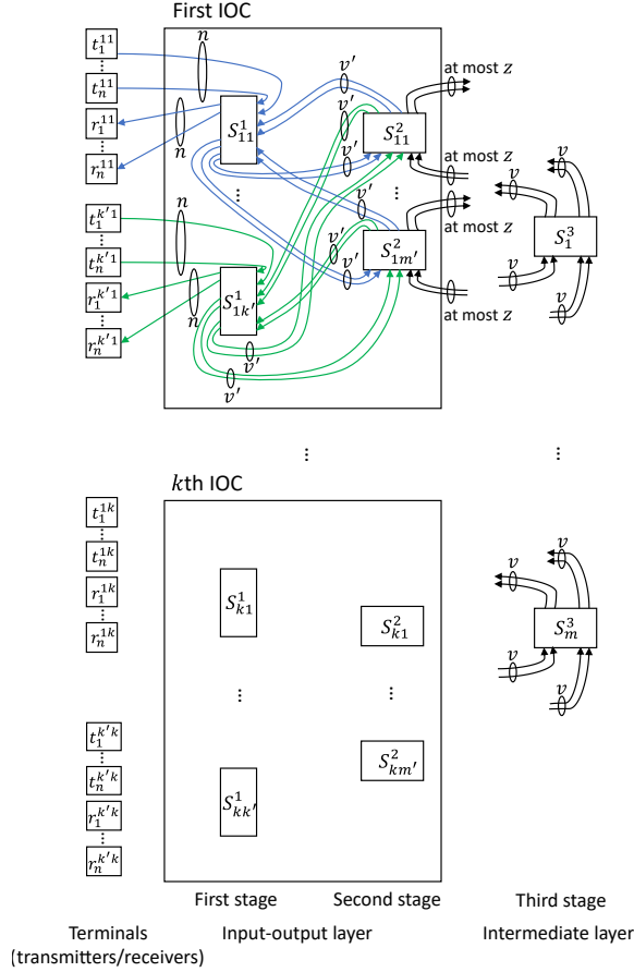
Fig. 3. Structure of 3TF.
