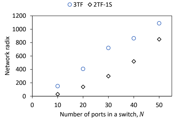
Fig. 4. Dependency of network radix on N with a = 200 and \epsilon = 0 .
