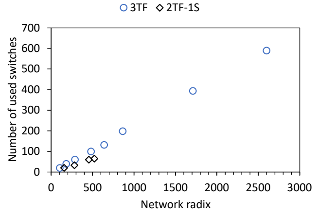
Fig. 14. Number of switches used depending on network radix with N = 40 and \epsilon = 0 .
