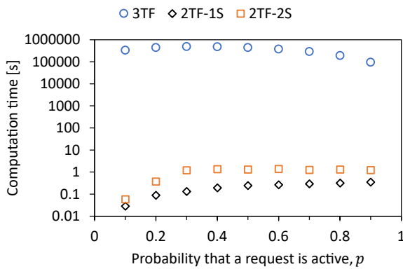
Fig. 13. Dependency of computation time on p with N = 40 , a = 2400 , and \epsilon = 0.1 .
