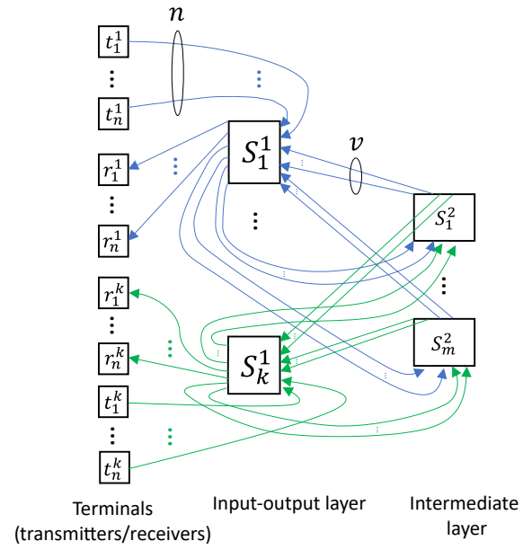
Fig. 2. Structure of two-stage TF-Clos (2TF). The input-output layer has k switches, each connecting n transmitters and n receivers. The intermediate layer has m switches. One side of each switch in the input-output layer connects one side of each switch in the intermediate layer with v links.
