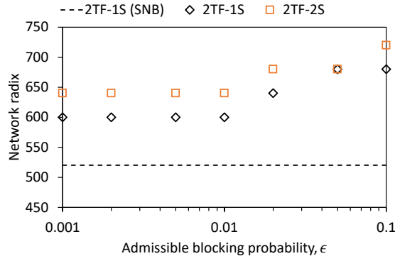
Fig. 8. Dependency of network radix on \epsilon with N = 40 , a = 2400 , and p = 0.5 for 2TF-1S and 2TF-2S.
