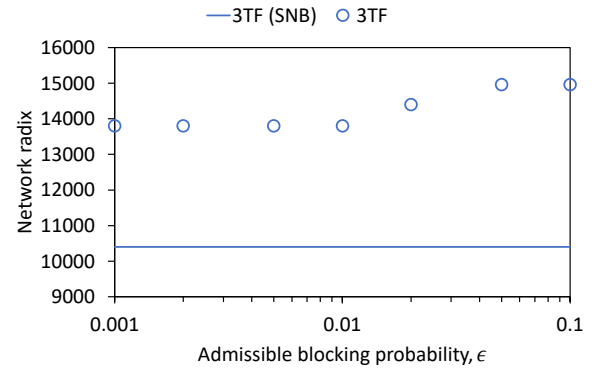
Fig. 7. Dependency of network radix on \epsilon with N = 40 , a = 2400 , and p = 0.5 for 3TF.
