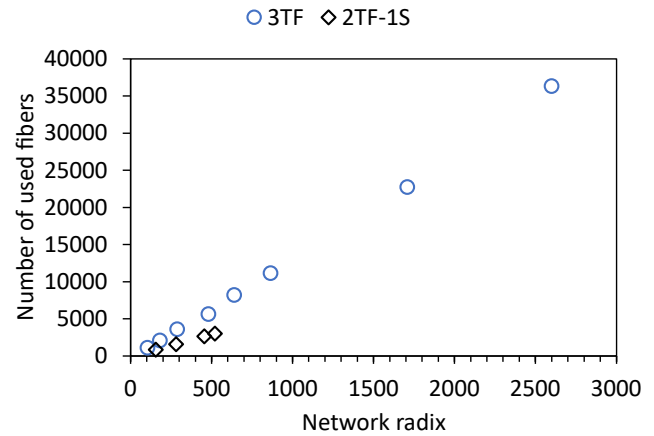
Fig. 15. Number of fibers used depending on network radix with N = 40 and \epsilon = 0 .
