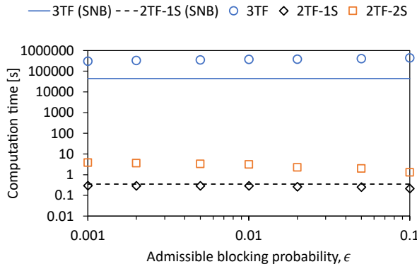
Fig. 12. Dependency of computation time on \epsilon with N = 40 , a = 2400 , and p = 0.5 .
