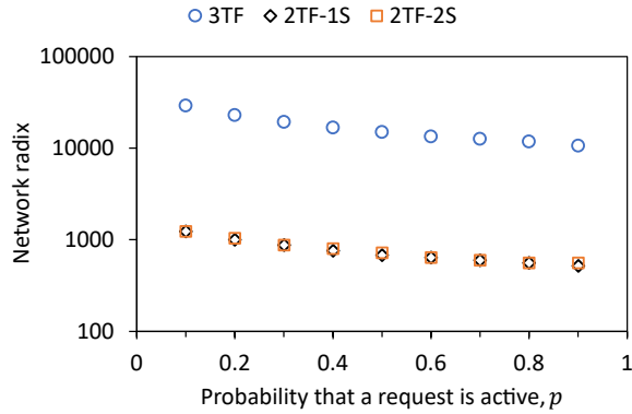
Fig. 9. Dependency of network radix on p with N = 40 , a = 2400 , and \epsilon = 0.1 .
