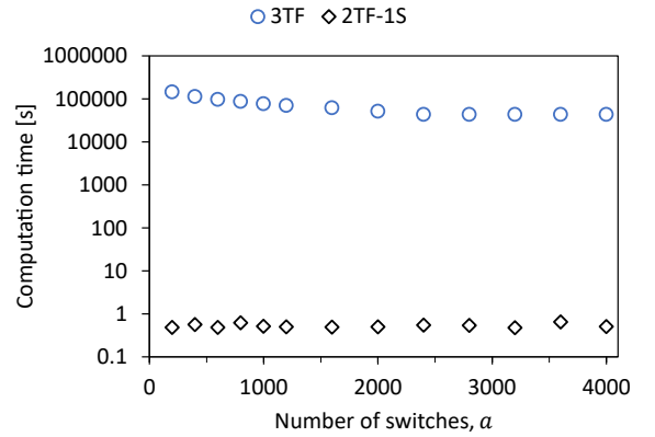
Fig. 11. Dependency of computation time on a with N = 40 and \epsilon = 0 .
