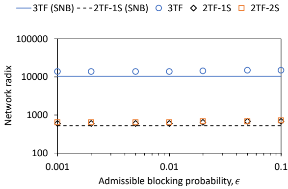
Fig. 6. Dependency of network radix on \epsilon with N = 40 , a = 2400 , and p = 0.5 .
