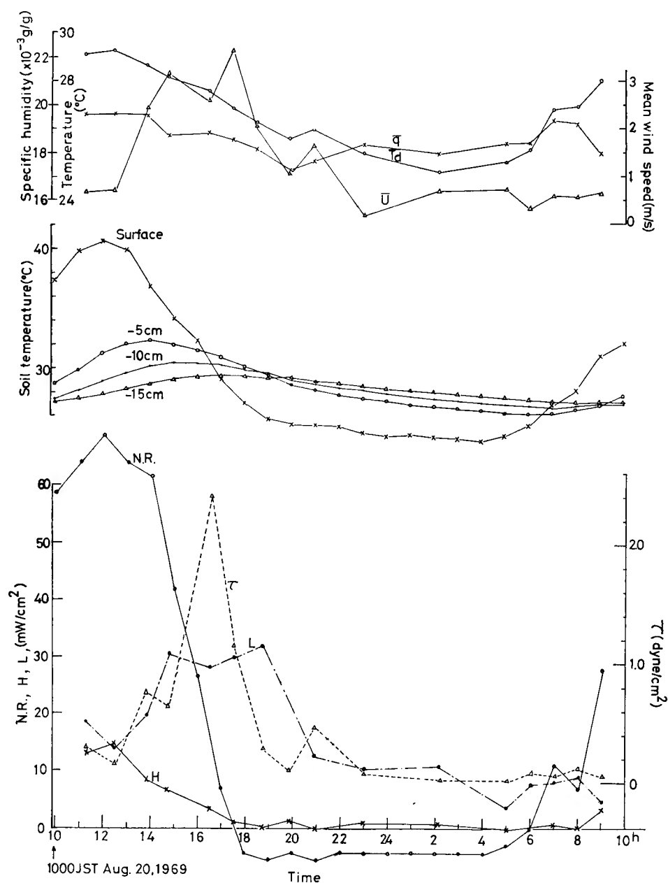
Fig. 4. An example of the time variations of vertical fluxes and mean quantities.
