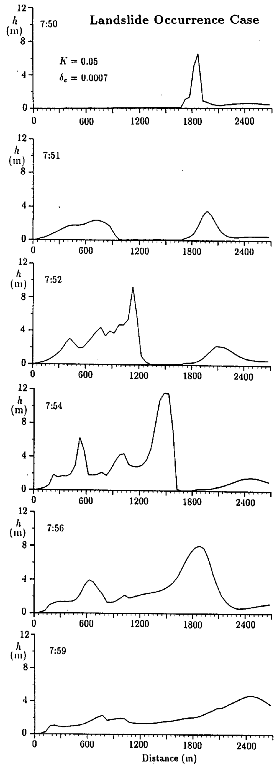
Fig. 8 Temporal variation of the flow depth along the channel (landslide occurrence case).
