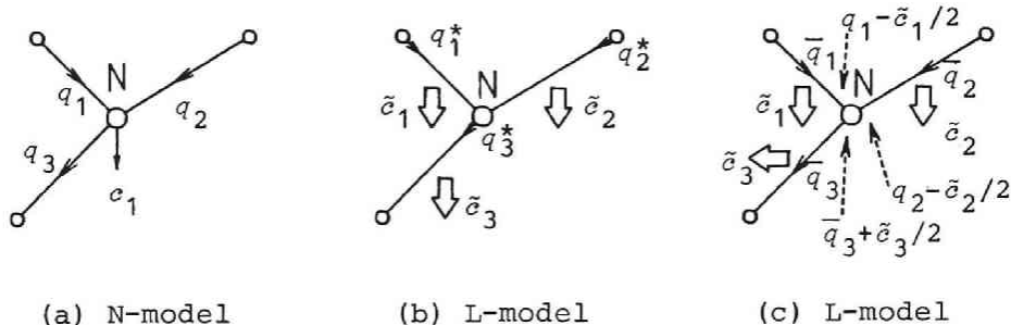
Fig. 4.2. Flow conservation law.
