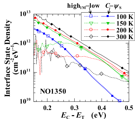
FIG. 7. Interface state densities of sample NO1350 evaluated by the C-\psi_s (solid line) and high 1M -low (broken line) methods at different measurement temperatures.
