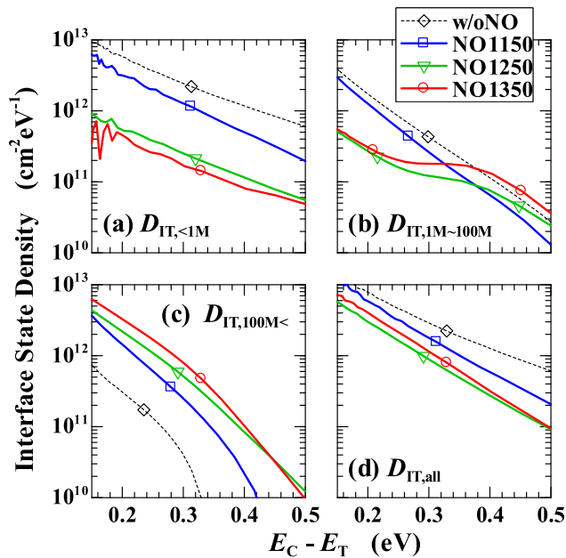
FIG. 4. Densities ( D_{IT,<1M} , D_{IT,1M\sim 100M} , and D_{IT,100M<} ) of interface states responding to a frequency range of (a) f < 1 MHz, (b) 1 \text{ MHz} < f < 100 \text{ MHz} , and (c) 100 \text{ MHz} < f , respectively, and (d) total interface state density ( D_{IT,all} ) for samples annealed in NO at different temperatures.
